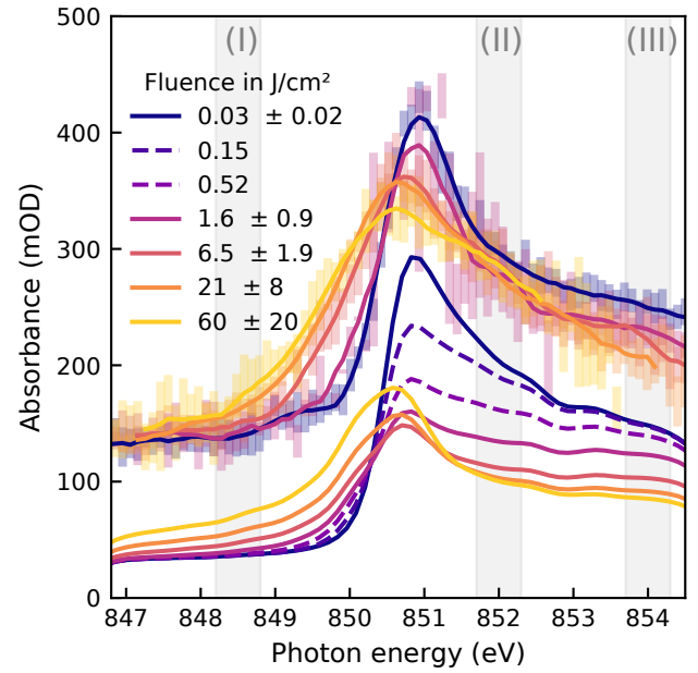
FIG. 3. Fluence-dependent Ni L_3 -edge spectra, measured (top) and simulated (bottom). The fluence of events contributing to each spectrum is given in terms of mean and standard deviation. Dashed simulated spectra do not have a corresponding measurement. The regions of interest from which absorbance changes shown in panels b), d), and e) of Fig. 4 were quantified are shaded and labeled (I), (II), and (III), respectively. The error bars are shown for the measured spectra and represent the 95% confidence intervals for each bin of 102 meV width; solid lines of the measured spectra are smoothed using a Savitzky-Golay filter using windows of 21 bins and 4th-order polynomials. The experimental spectra are vertically offset by 100 mOD.
