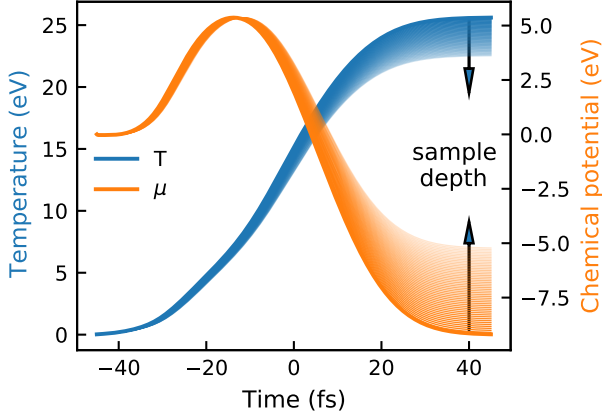
FIG. 7. Temperature and chemical potential over time for a pulse at 857.5 \text{ eV} with a pulse energy of 30 \text{ J/cm}^2 . The solid line represents the properties at the sample surface and the thin lines represent the deeper layers that are exposed to less X-ray fluence, as indicated by arrows and increasing transparency.
