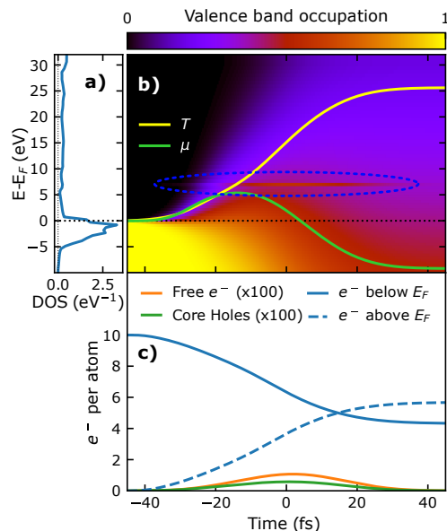
FIG. 5. Evolution of electronic populations (simulation) in a single voxel at the sample surface for a pulse of 858.3 eV, with a pulse energy of 30 J/cm 2 . Panel a) shows the total DOS used as an input for the simulation. Panel b) shows the energy-resolved occupation (between 0 and 1) of the valence band over time, relative to the Fermi energy, and shares the corresponding axes with panels a) and c). The population (in electrons/atom/eV) is the product of the DOS and the occupation. The thermalized valence occupation lags a few femtoseconds behind the current chemical potential \mu ; the temperature T of the valence system rises rapidly, ultimately reaching up to 25 eV. The bleaching of valence states (highlighted with a blue dotted ellipse) is visible as a high non-thermal population at the resonant photon energy around 7 eV above the Fermi level. Panel c) shows the number of core holes and free electrons over time, as well as the number of electrons in the valence system below and above the Fermi energy.
