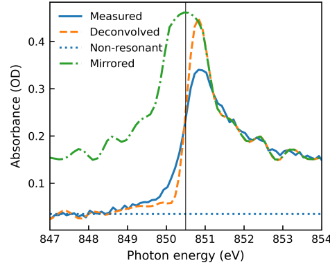
FIG. 9. Derivation of absorption lengths as input parameters , reconstructed from a measured ground-state spectrum (blue line). The non-resonant absorption level (blue dots) was determined from the pre-edge region. The measured resonant absorption length was deconvolved with the experimental resolution (orange dashes) and mirrored around the rising edge to retrieve a symmetric resonant absorption length around the resonance (green dot-dashed line). See main text for details.
