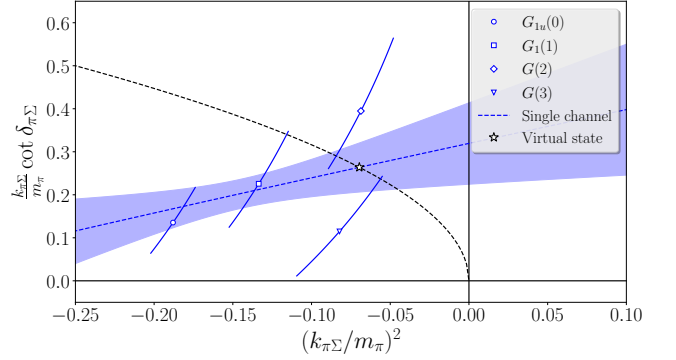
FIG. 4. The elastic \pi\Sigma amplitude near threshold. The points are obtained from Eq. (1) using a single channel and \ell_{\text{max}} = 0 . The shaded band denotes a fit of the four levels shown to a two-parameter effective range expansion. A pole on the real axis in the second Riemann sheet (a virtual bound state) occurs when k_{\pi\Sigma} \cot \delta_{\pi\Sigma} - ik_{\pi\Sigma} = 0 below threshold. This is where the black dashed line intersects the fit.
