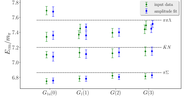
FIG. 3. Finite-volume spectrum in the center-of-mass frame used as input data to constrain parametrizations of the coupled-channel \pi\Sigma - \bar{K}N scattering amplitude. Each column corresponds to a particular irrep \Lambda(\mathbf{d}^2) of the little group of total momentum \mathbf{P}^2 = (2\pi/L)^2 \mathbf{d}^2 . Only irreps where the \ell = 0 partial wave contributes are included. Dashed lines indicate various thresholds, as labeled. Model energies from the resultant scattering-amplitude fit are given by blue squares.
