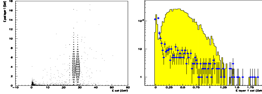
Figure 2: Left: the energy on the first Si pad plane vs. total energy on the calorimeter for electrons of 30 GeV (boxes) and pions of 75 GeV (dots). Right: energy response to 30 GeV electrons (histogram) and 30 GeV pions (dots) on the first longitudinal segmentation of the calorimeter. The peak at low energy on the histogram is due to a contamination of the electron beam.
