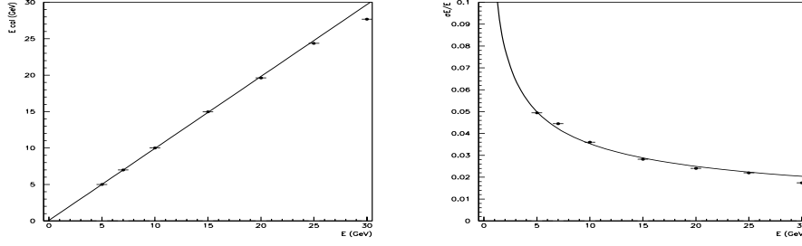
Figure 1: Left: detector energy response to electrons of different energy. Right: energy resolution as a function of the input energy in GeV. The full line corresponds to the fitted function \sigma_E/E = 11.1\%/\sqrt{E} . The point at 30 GeV was excluded from the fit.
