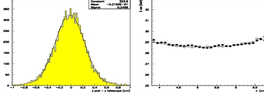
Figure 3: Left: the difference y_{\text{reconstructed}} - y_{\text{telescope}} for the vertical ( y ) coordinate on the first Si pad plane for 10 GeV electrons. Right: energy dependence on the horizontal ( x ) impact coordinate for 30 GeV electrons: predicted by the telescope (open circles), reconstructed by the first plane of Si pads (black dots).
