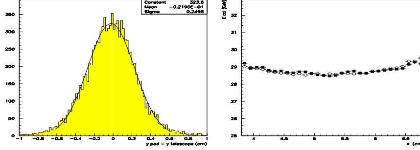
Figure 3: Left: the difference y_{\text{reconstructed}} - y_{\text{telescope}} for the vertical ( y ) coordinate on the first Si pad plane for 10 GeV electrons. Right: energy dependence on the horizontal ( x ) impact coordinate for 30 GeV electrons: predicted by the telescope (open circles), reconstructed by the first plane of Si pads (black dots).
