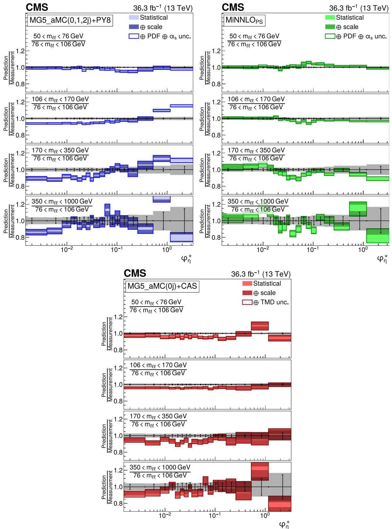
Fig. 23 Ratios of differential cross sections in \phi_n^*(\ell\ell) for invariant m_{\ell\ell} with respect to the peak region 76 < m_{\ell\ell} < 106 GeV. Compared to model predictions from MG5_aMC (0, 1, and 2 jets at NLO) + PYTHIA
