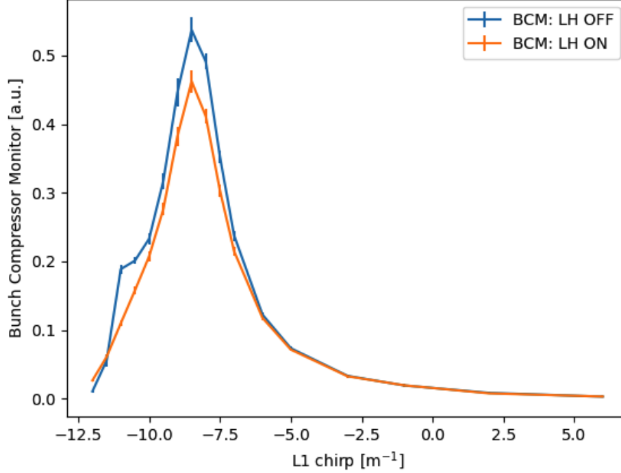
FIG. 9: Signal from Bunch Compressor Monitor after the last bunch compressor BC2.
