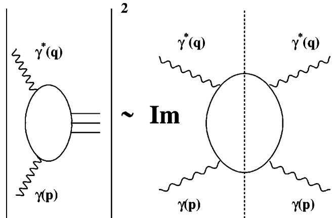
FIG. 1. The cross section for the \gamma^*\gamma \rightarrow \text{hadrons} scattering and its relation to the imaginary part of the forward \gamma^*\gamma \rightarrow \gamma^*\gamma amplitude.
