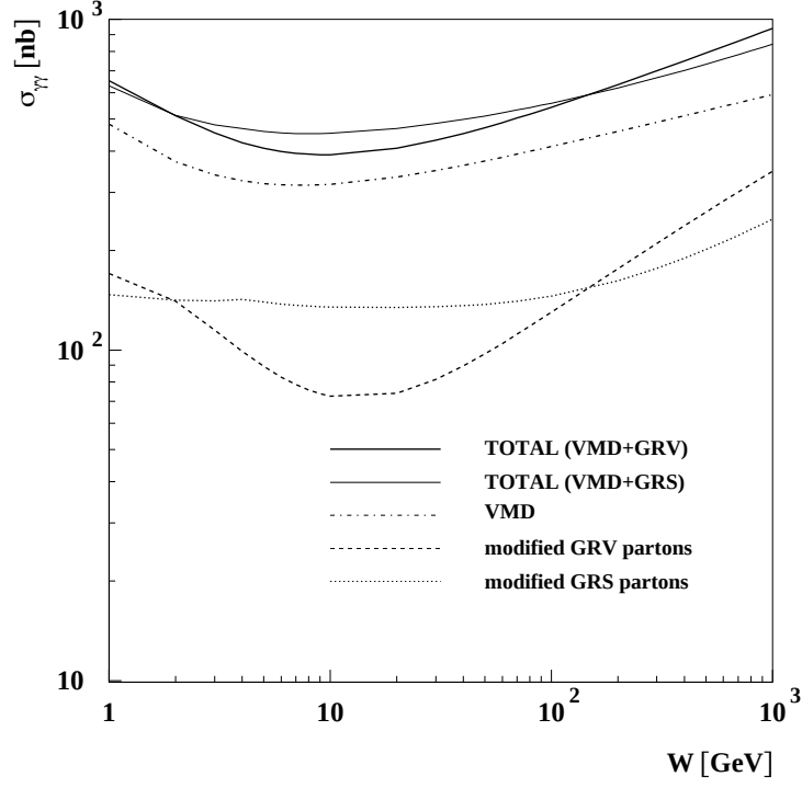
Figure 9: The total \gamma\gamma cross-sections \sigma_{\gamma\gamma}(W) (continuous lines) calculated from equation (15) and plotted in a wide energy range which includes the region that will be accessible in future linear colliders. Shown separately are the VMD and partonic components of \sigma_{\gamma\gamma}(W) . They correspond to the first and the second term of the r.h.s. of equation (15) respectively. Partonic contributions were obtained using two different parametrizations of F_2^{\text{QCD}} .
