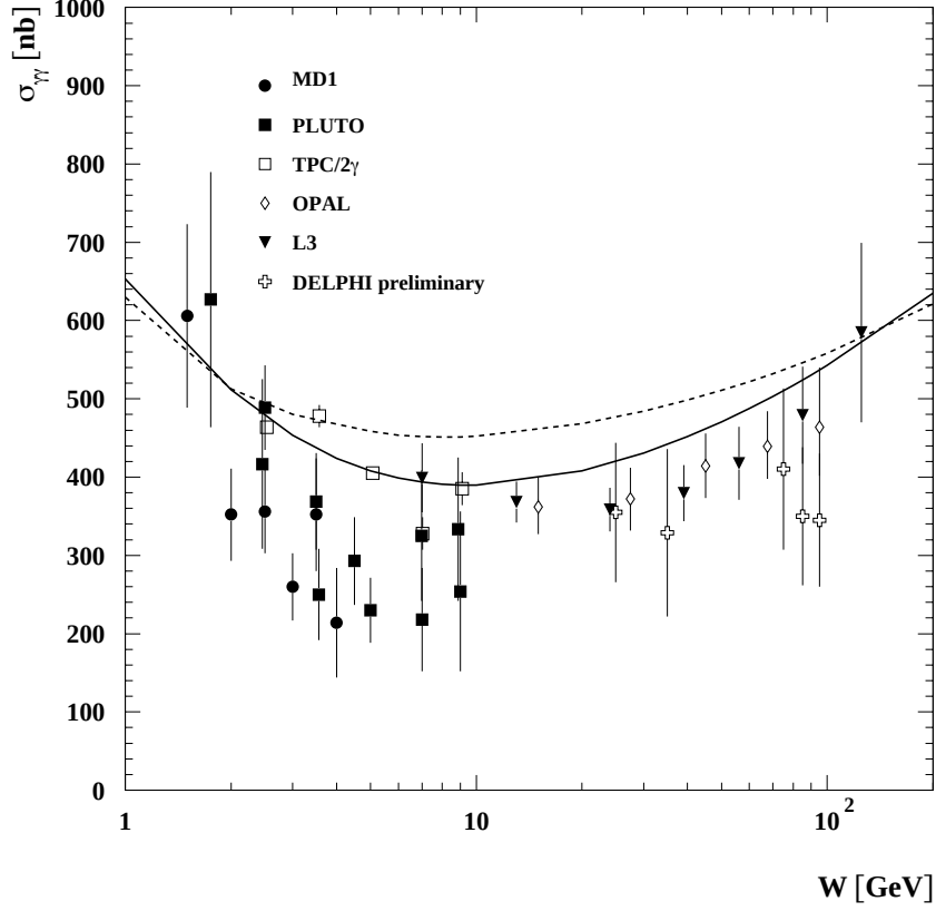
Figure 8: Comparison of our predictions for \sigma_{\gamma\gamma}(W) based on equation (15) with experimental results [30, 31, 32, 33, 34, 35]. The curves correspond to different LO parametrizations of F_2^{\text{QCD}} : GRV [19] (solid line) and GRS' [20] (dashed line). Error bars correspond to statistical and systematic errors added in quadrature.
