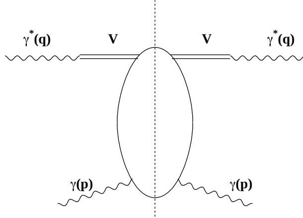
Figure 4: Diagrammatic representation of the VMD model in the \gamma^*\gamma scattering.
