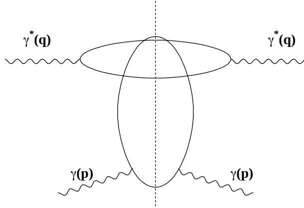
Figure 5: Diagrammatic representation of the dispersion relation.
