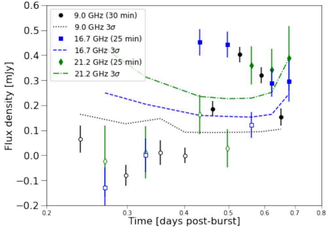
Figure 2. Lower cadence radio light curves of GRB 210702A at 9.0 (30 min), 16.7 (25 min) and 21.2 GHz (25 min) to demonstrate the late-time detections are significant compared to the less sensitive early-time data and therefore indicative of transient behaviour. Filled data points are considered detections ( \text{SNR} \geq 3 ) whereas the hollow circles are force-fitted flux density values ( \text{SNR} < 3 ). The dashed, dash-dotted and dotted lines represents the detection threshold at each of the three plotted frequencies (marked as an \text{SNR} of 3).
