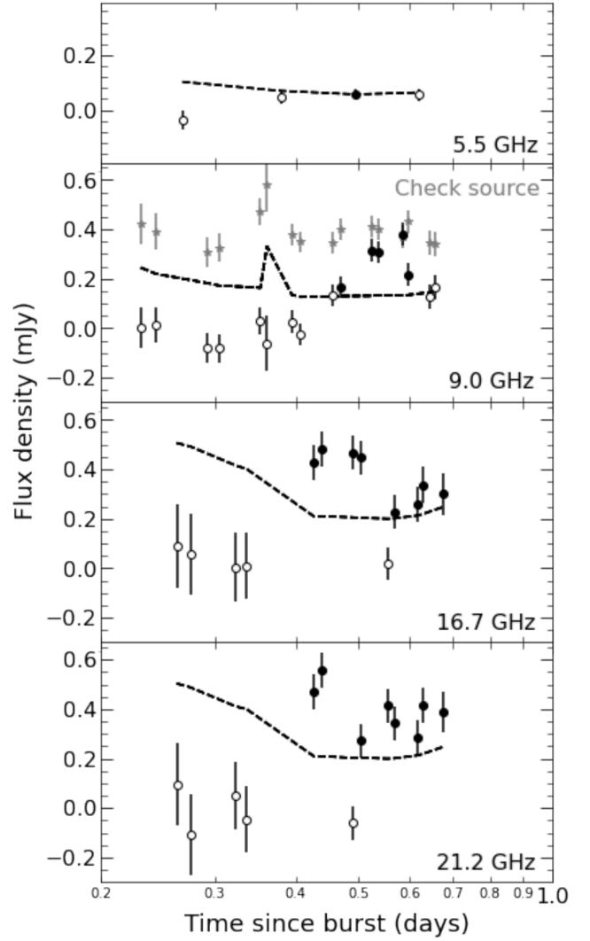
Figure 1. Radio light curves of GRB 210702A at 5.5 (60 min bins), 9.0 (15 min), 16.7 (12.5 min) and 21.2 GHz (12.5 min). Filled data points are considered detections ( \text{SNR} \geq 3 ) whereas the hollow circles are force-fitted flux density values ( \text{SNR} < 3 ). The dashed line represents the detection threshold (marked as an SNR of 3). At 9.0 GHz we also plot the flux density of a check source in the field to demonstrate that the observed transient nature of what we have identified as the radio afterglow to GRB 210702A was not an instrumental artefact.
