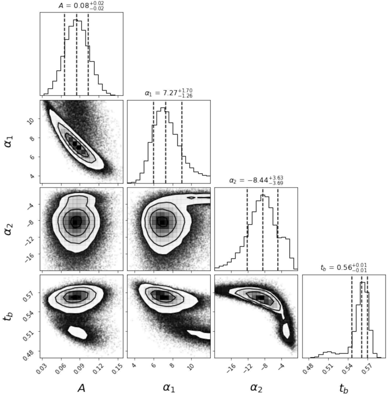
Figure B1. Corner plot for the model posterior sample from the broken power law fitted to the 9.0 GHz light curve using the MCMC method with 10,000 step production chains for all of the 20 walkers assuming uniform priors for all four parameters. The plotted parameter A is the amplitude, \alpha_1 is spectral index 1, \alpha_2 is spectral index 2, and t_b is the break time (see Equation 1 and Section 3.1). The three solid contour lines on the joint distribution panels correspond to 1, 2, and 3\sigma highest density intervals. The dashed lines on the marginal distribution panels show the 0.16, 0.5, and 0.84 quantiles (median and borders of a 1\sigma credible interval) for each parameter.
