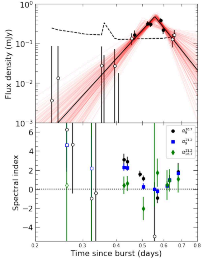
Figure 3. Top: Broken power law fit to the 9.0 GHz light curve. Data points are the same as for Figure 1. The red lines show a random selection of 200 out of 5000 trace samples from the MCMC model fitting. See the corresponding corner plots in Figure B1. Bottom: Radio spectral index temporal evolution between frequency pairs 9.0/16.7 GHz, 9.0/21.2 GHz, and 16.7/21.2 GHz. The broken powerlaw model traces of the 9.0 GHz light curve were used to interpolate the 9.0 GHz flux to the time of the 16.7 and 21.2 GHz observations. Filled data points are spectral indices calculated using the detections ( \text{SNR} \geq 3 ) at 16.7 and 21.2 GHz whereas open circles show the spectral index calculated using the force-fitted flux density values ( \text{SNR} < 3 ).
