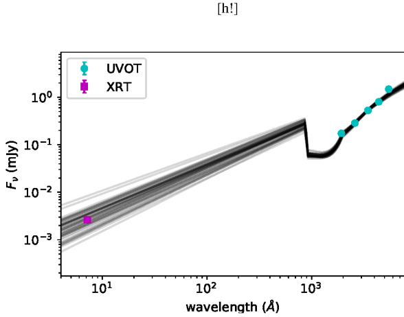
Figure 4. The optical-to-X-ray SED spectral fits for F_\nu (mJy) as a function of wavelength ( \text{\AA} ) for the Swift -XRT and -UVOT data at T_0 + 14370 s. This log-log plot shows the final position of each of the 50 walkers for a Gaussian spectral index prior as described in Section 3.3. See the corresponding corner plots in Figure B2.
