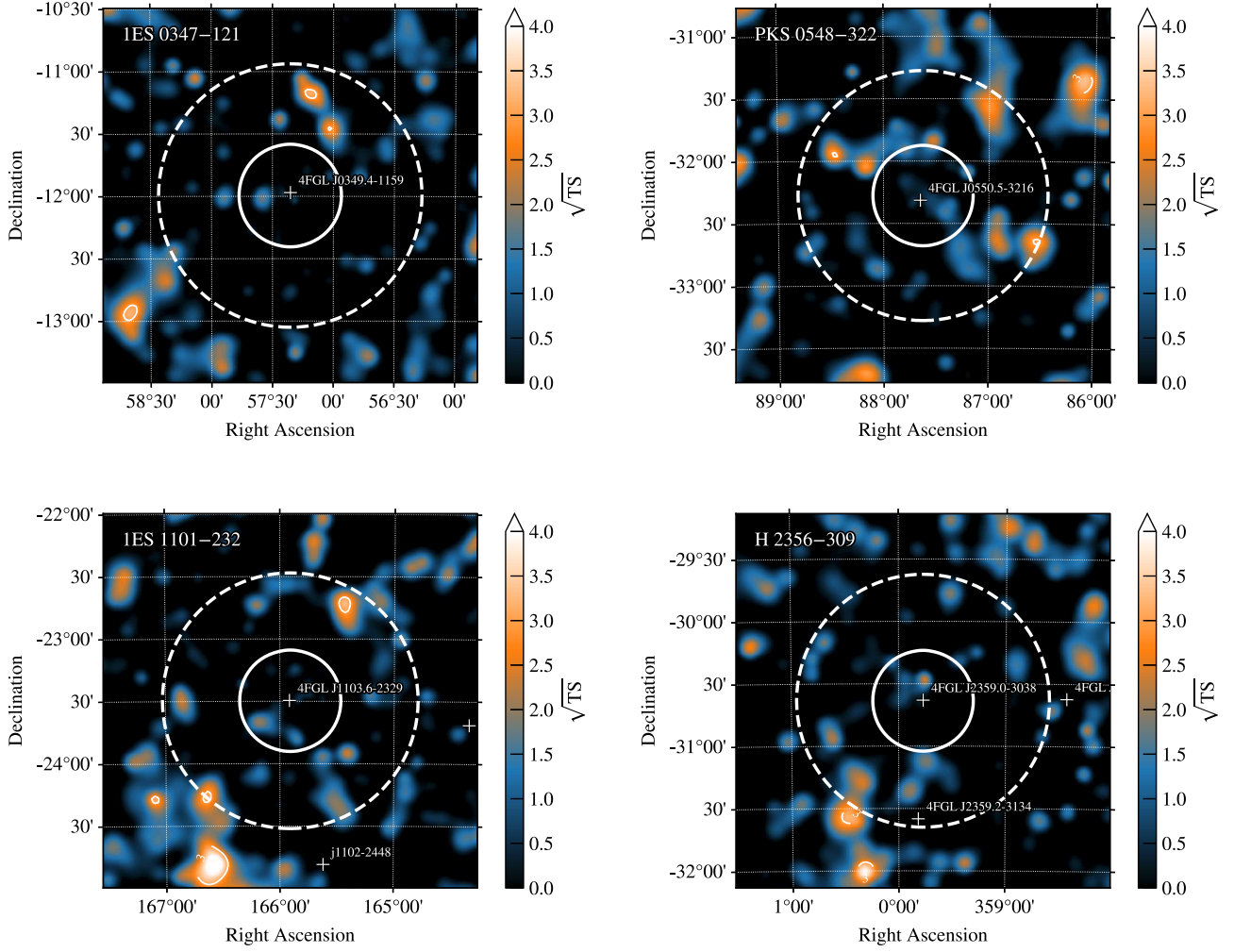
Figure 5. TS maps as in Figure 1 for all other considered sources. Again, no significant excess is observed close to any considered source. The additional source in the ROI of 1ES 1101–232 is marked with a lowercase j and its coordinates.
