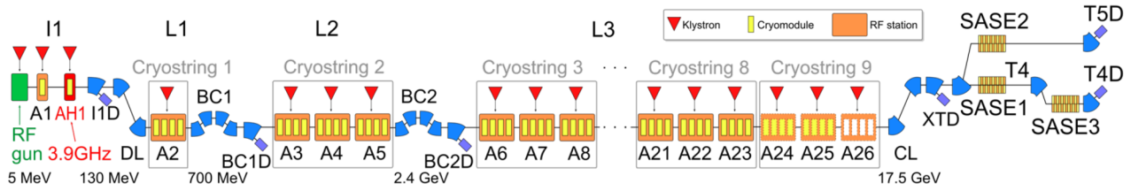
Figure 1: Schematic view of the RF stations, cryo strings and the accelerator sections of the European XFEL.
