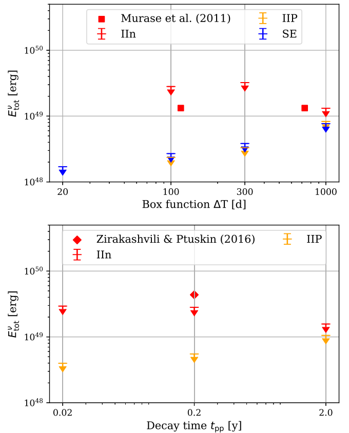
Figure 2. Upper limits on total neutrino ( \nu_{\mu} + \bar{\nu}_{\mu} ) energy assuming a box-like neutrino light curve (upper panel) and assuming a L_{\nu} \propto \left(1 + \frac{t}{t_{\text{pp}}}\right)^{-1} neutrino light curve as predicted by Zirakashvili & Ptuskin (2016). The energy ranges are the same as indicated in Figure 3. The model predictions by Murase et al. (2011) and Zirakashvili & Ptuskin (2016) are shown as red squares for comparison.
