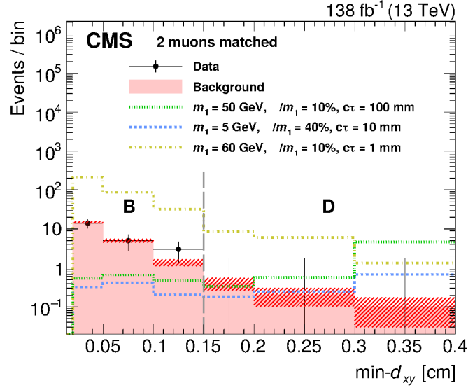
Figure 3: Measured \min-d_{xy} distribution in the 2-match category, after requiring the \min-d_{xy} muon to pass the isolation requirement I_{\text{PPF}}^{\text{rel}} < 0.25 (i.e., the B and D bins of the ABCD plane). Overlaid with a red histogram is the background predicted from the region of the ABCD plane failing the same requirement (the A and C bins), as well as three signal benchmark hypotheses (as defined in the legends), assuming \alpha_{\text{D}} = \alpha_{\text{EM}} (the fine-structure constant). The red hatched bands correspond to the background prediction uncertainty. The last bin includes the overflow.
