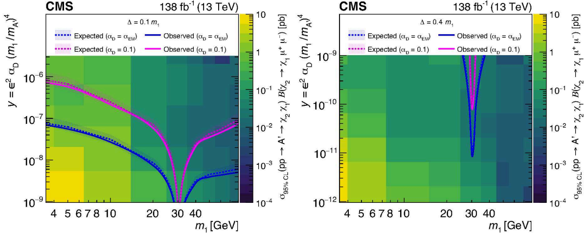
Figure 4: Two-dimensional observed limits on \sigma(pp \rightarrow A' \rightarrow \chi_1\chi_2) \mathcal{B}(\chi_2 \rightarrow \chi_1\mu^+\mu^-) , for \Delta = 0.1 m_1 (left) and 0.4 m_1 (right), as functions of the DM mass m_1 and the interaction strength y , with m_{A'} = 3 m_1 . Solid (dashed) curves denote the observed (expected) exclusion limits at 95% CL, with 68% CL uncertainty bands around the expectation. Regions above the curves are excluded, depending on the \alpha_D hypothesis: \alpha_D = \alpha_{EM} (dark blue) or 0.1 (light magenta).
