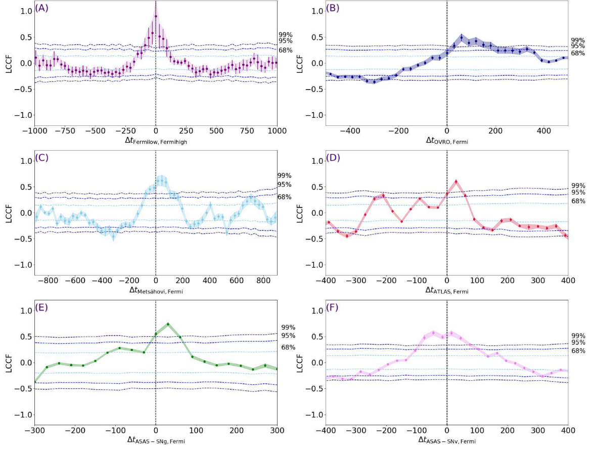
Figure 5. Local cross-correlation functions (LCCFs) calculated between the different lightcurves are shown in color. The x-axis represents the time delay, \Delta t_{a,b} = t_a - t_b , in days for two lightcurves a and b . The dashed vertical line corresponds to \Delta t_{a,b} = 0 . The corresponding shaded regions indicate the error bounds of the LCCFs. The blue lines represent the 68%, 95% and 99% confidence intervals (from lighter to darker shades) derived from Monte Carlo simulations.
