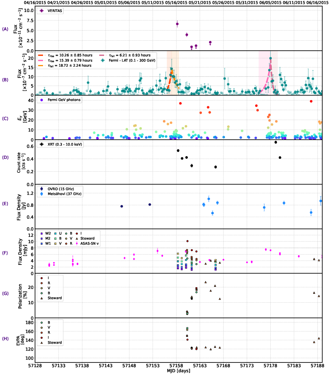
Figure 3. Multiwavelength lightcurves of S3 1227+25 between MJD 57128 and MJD 57189, which corresponds to midnight on April 16, 2015 until midnight on June 16, 2015, a month either side of the VERITAS detection. (A) Daily-binned VHE lightcurve for VERITAS observations above an energy threshold of 120 GeV. Upper limits at 95% confidence level are quoted for observations with a significance of lower than 2\sigma . (B) Fermi-LAT lightcurve in 6 hour bins in the 0.1–300 GeV band. The shaded regions indicate the two periods of flaring activity used to compute the variability timescales, obtained from the fits (dashed curves) and shown in legend. Upper limits are shown for individual bins having a significance of lower than 2\sigma . (C) Fermi-LAT GeV photon energies positionally coincident (at 95% containment) with the source position. (D) Swift -XRT count rate in the 0.3–10 keV band. (E) Radio flux observations: OVRO (dark blue) and Metsähovi (light blue) lightcurves at 15 GHz and 37 GHz respectively. (F) Optical/UV flux observations: Swift -UVOT (square markers), Lowell Observatory (circles), Steward photometry in the 4000–7000 Å band (triangles) and optical data, not corrected for extinction, from the ASAS-SN Sky Patrol (magenta points). (G) Electric vector polarization angle (EVPA): Lowell Observatory (circles), Steward photometry in the 4000–7000 Å band (triangles). (H) Polarization: Lowell Observatory (circles), and Steward photometry in the 4000–7000 Å band (triangles).
