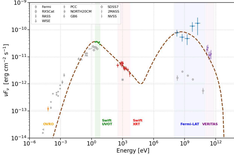
Figure 6. The multiwavelength broadband SED of S3 1227+25 during the nights of the VERITAS detection, May 16 – May 18, 2015 (MJD 57158 – 57160), fitted using agnpy . The grey points represent archival data. The dashed brown curve represents the best fit one-zone synchrotron and SSC radiation model, obtained using all of the 5000 samples from all of the 30 walkers, with the parameters shown in Table 2.
