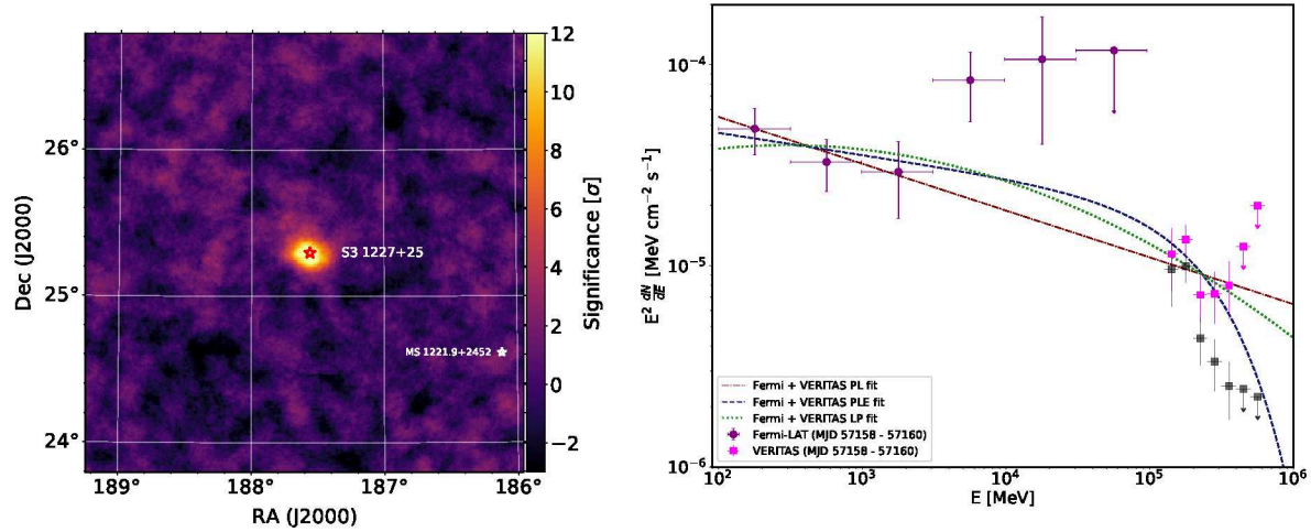
Figure 2. Left: VERITAS significance skymap based on observations taken on May 16, 2015 and May 18, 2015 UTC (MJD 57158 and 57160) at the location of the new VHE source positionally coincident with S3 1227+25. The known VHE blazar MS 1221.9+2452, shown with a white marker, was not detected during this period. Right: The purple data points show the Fermi -LAT spectrum obtained for S3 1227+25 in the energy range 100 MeV–100 GeV between May 16 and May 18, 2015 UTC (MJD 57158 – 57160). The data are binned into two energy bins per decade, with individual bins having a TS < 4 (roughly corresponding to a significance of \sim 2\sigma ) considered as upper limits. The magenta data points show the VHE spectrum for S3 1227+25 based on VERITAS observations taken on May 16 and May 18, 2015 UTC (MJD 57158 – 57160). A minimum significance of two standard deviations and three on-source photons are required for each flux point and upper limits at 95% confidence level are quoted otherwise. De-absorbed flux points, using the Domínguez et al. (2011) EBL model, are shown in magenta and the corresponding observed fluxes are shown in black. A power law (PL), power law with exponential cut-off (PLE) and log parabola (LP) function is fit to the de-absorbed combined gamma-ray spectrum and is shown as dashed red, blue and green curves respectively.
