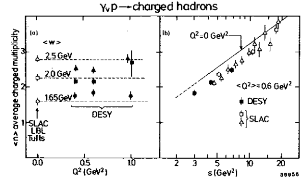
Fig. 2: Average charged multiplicity (a) as a function of Q^2 and (b) as a function of W^2 = s . The full symbols refer to data from ref. 5. The measurements at Q^2 = 0 GeV 2 (in (b) drawn as solid line) were extracted from ref. 4. The open squares and triangles represent results from ref. 6 and 7 respectively.
