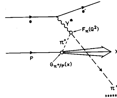
Fig. 15: Diagram of electron scattering from virtual pions pre-existing in the target proton.
