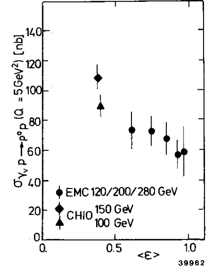
Fig. 17: Total cross section for exclusive \rho^0 electroproduction as a function of \varepsilon . The data stem from EMC 52 and CHIO 53 .
