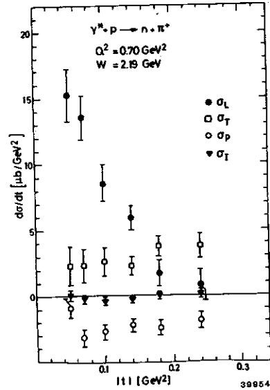
Fig. 14: d\sigma/dt for electroproduction of \pi^+n as a function of |t| . The contributions due to the various helicities and polarisations of the virtual photons are separated 44 .
