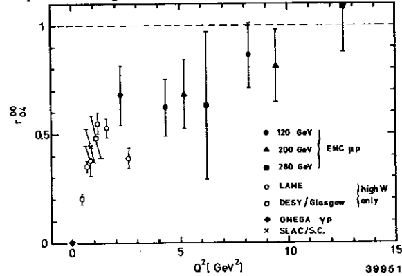
Fig. 18: \rho^0 density matrix element r_{00}^{04} . Results from various experiments are shown: EMC 52 , LAME 54 , DESY-Glasgow 56 , SLAC 57 , OMEGA 58 .
