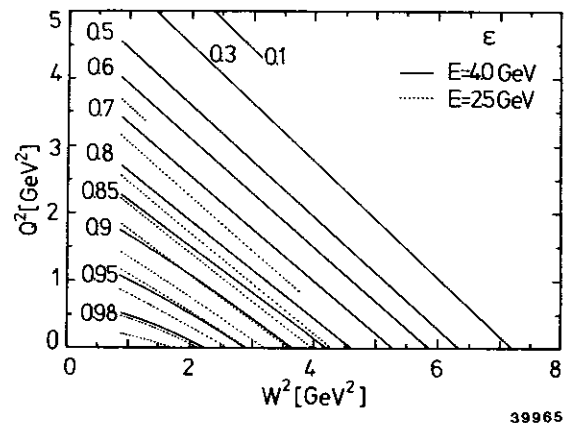
Fig. 21: Contours of \epsilon in the Q^2 - W^2 plane. The solid lines refer to the beam energy of 4 GeV, the dotted lines to 2.5 GeV. The values of \epsilon are the same for both energies but only the 4 GeV lines are labelled.
