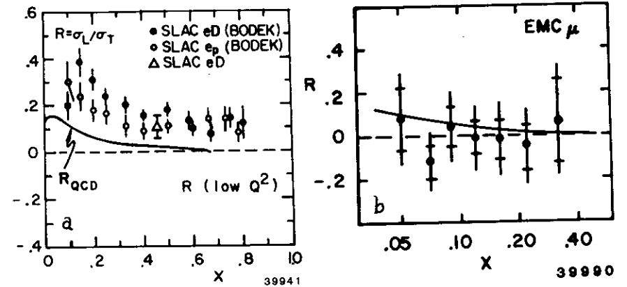
Fig. 13: R = \sigma_L/\sigma_T as a function of x : (a) at low Q^2 ( \leq 10\text{GeV}^2 ) 43 and (b) at high Q^2 ( \geq 10\text{GeV}^2 ) 42 . The leading order QCD predictions (solid lines) are discussed in references 42 and 43 respectively.
