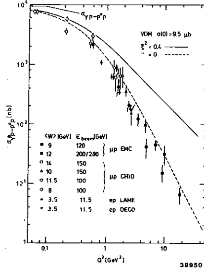
Fig. 16: Total cross section for exclusive \rho^0 electroproduction as a function of Q^2 . The data are taken from measurements carried out by the following collaborations: EMC 52 , CHIO 53 , LAME 54 , DECO 55 . The lines represent VMD calculations 50 with different values of the parameter \xi^2 .
