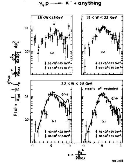
Fig. 4: Inclusive \pi^- structure function 5 as a function of x_F in different W and Q^2 intervals. In (d) contributions from the reaction ep \rightarrow epp^0 are removed. The solid lines in (c) and (d) represent data from ref. 15.
