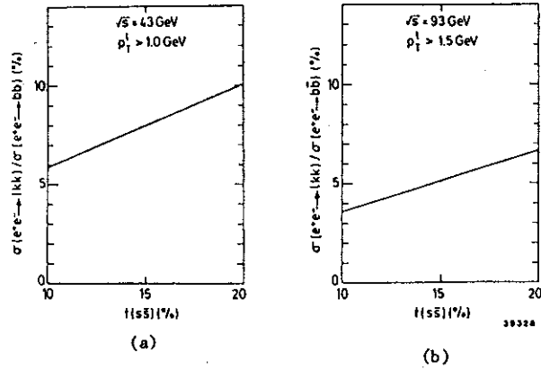
Fig 23: \sigma(e^+e^- \rightarrow l\bar{l}K\bar{K})/\sigma(e^+e^- \rightarrow b\bar{b}) summed over all charged combinations of l^\pm and K^\pm as a function of f(ss) with the indicated cuts. Note that (l\bar{l}K\bar{K}) belong to the same hemisphere (jet) (from ref. 21).
