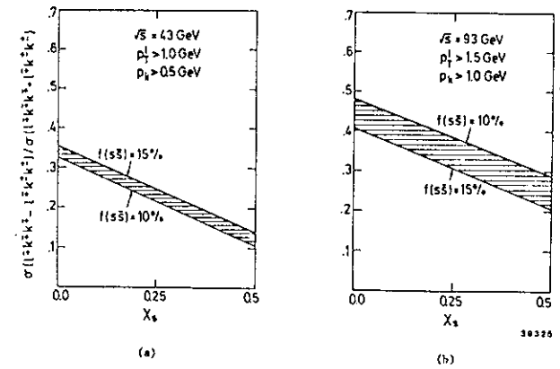
Fig 21: The ratio R(KK) = [\sigma(e^+e^- \rightarrow l^+l^-K^+K^-X) - \sigma(e^+e^- \rightarrow l^+l^-K^+K^-X)] / [\sigma(e^+e^- \rightarrow l^+l^-K^+K^-X) + \sigma(e^+e^- \rightarrow l^+l^-K^+K^-X)] as a function of the weak mixing measure, with the indicated values of the parameters (from ref. 21).
