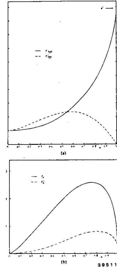
Fig 2: The coefficients \gamma_{tot} (= R_V^q) , \gamma'_{tot} (= R_A^q) , \gamma_F and \gamma'_F for the cross sections \sigma_q and \Delta_q as functions of \mu ( \mu = quark mass/beam energy) (from ref. 33).
