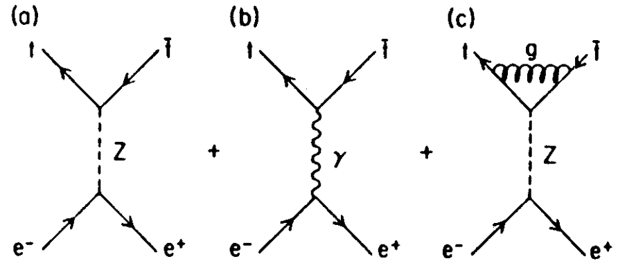
Fig 9: Feynman diagrams contributing to the normal polarization P_N of the top quark in e^+e^- \rightarrow Z^0, \gamma \rightarrow t\bar{t} (a) Z^0 -exchange Born graph (b) \gamma -exchange Born graph (c) Z^0 -exchange including QCD corrections.
