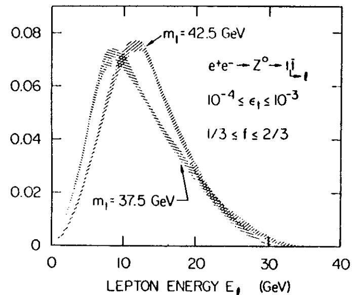
(c) Dependence on polarization and fragmentation effects. The shaded areas indicate bounds of the lepton energy distribution for the values of the parameters in the indicated range.
