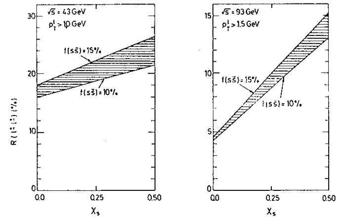
Fig 22: The dilepton ratio R = (N^{++} + N^{--}) / (N^{++} + N^{--} + N^{+-} + N^{-+}) with the indicated values of the parameter (from ref. 21)
