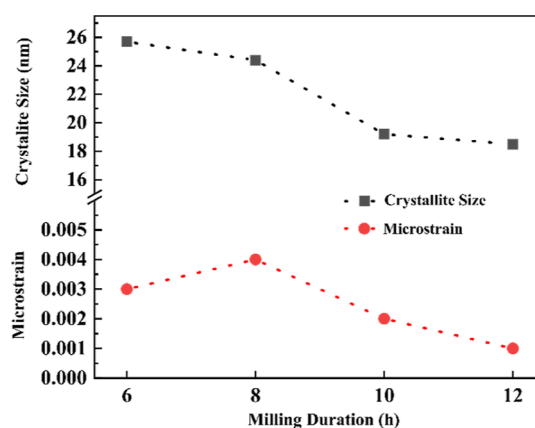
Figure 12. Variation of crystallite size and microstrain with respect to milling durations.
