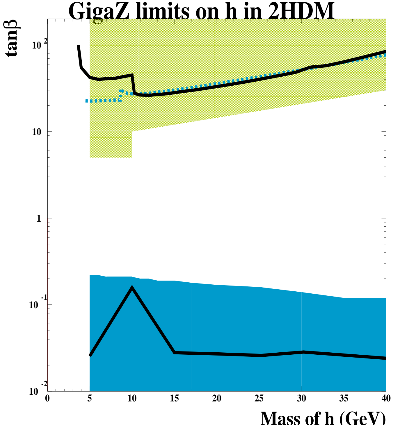
Figure 2: Potential exclusion range at GigaZ for the light scalar h as a function of its mass and \tan\beta (for \sin(\beta - \alpha)=0 ). The upper light (green) shaded region is excluded by the Yukawa process, the lower dark (blue) shaded region due to Z \rightarrow h\gamma . The upper limit from Z \rightarrow h\gamma for \tan\beta > 1 is indicated by the (blue) dotted line. Also shown is the current best limits obtained at LEP (black lines - upper from the Yukawa process and lower from the radiative Z decay).
