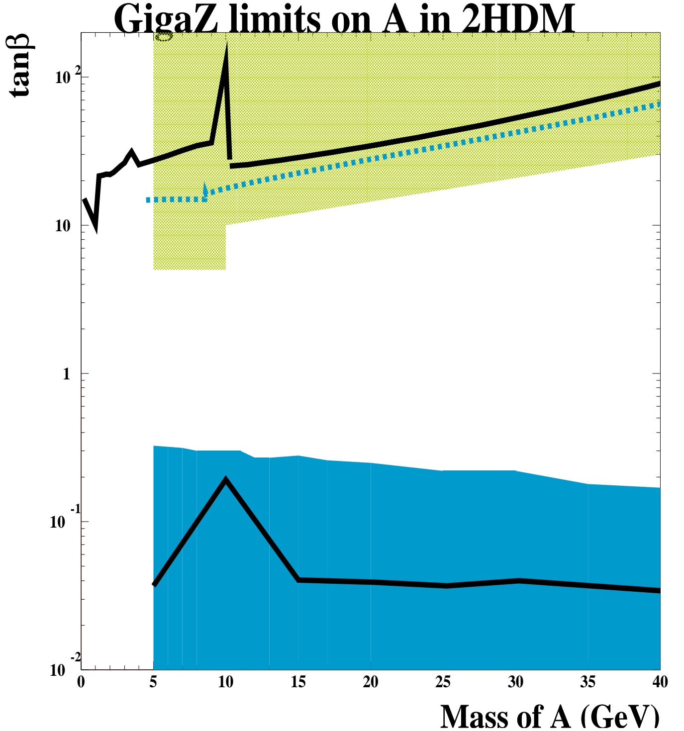
Figure 3: Potential exclusion range at GigaZ for the light scalar A as a function of its mass and \tan\beta . The upper light (green) shaded region is excluded by the Yukawa process, the lower dark (blue) shaded region due to from Z \rightarrow A\gamma . The upper limit from Z \rightarrow A\gamma for \tan\beta > 1 is indicated by the (blue) dotted line. Also shown is the current best limits obtained at LEP (black lines- upper from the Yukawa proces and lower from the radiative Z decay).
