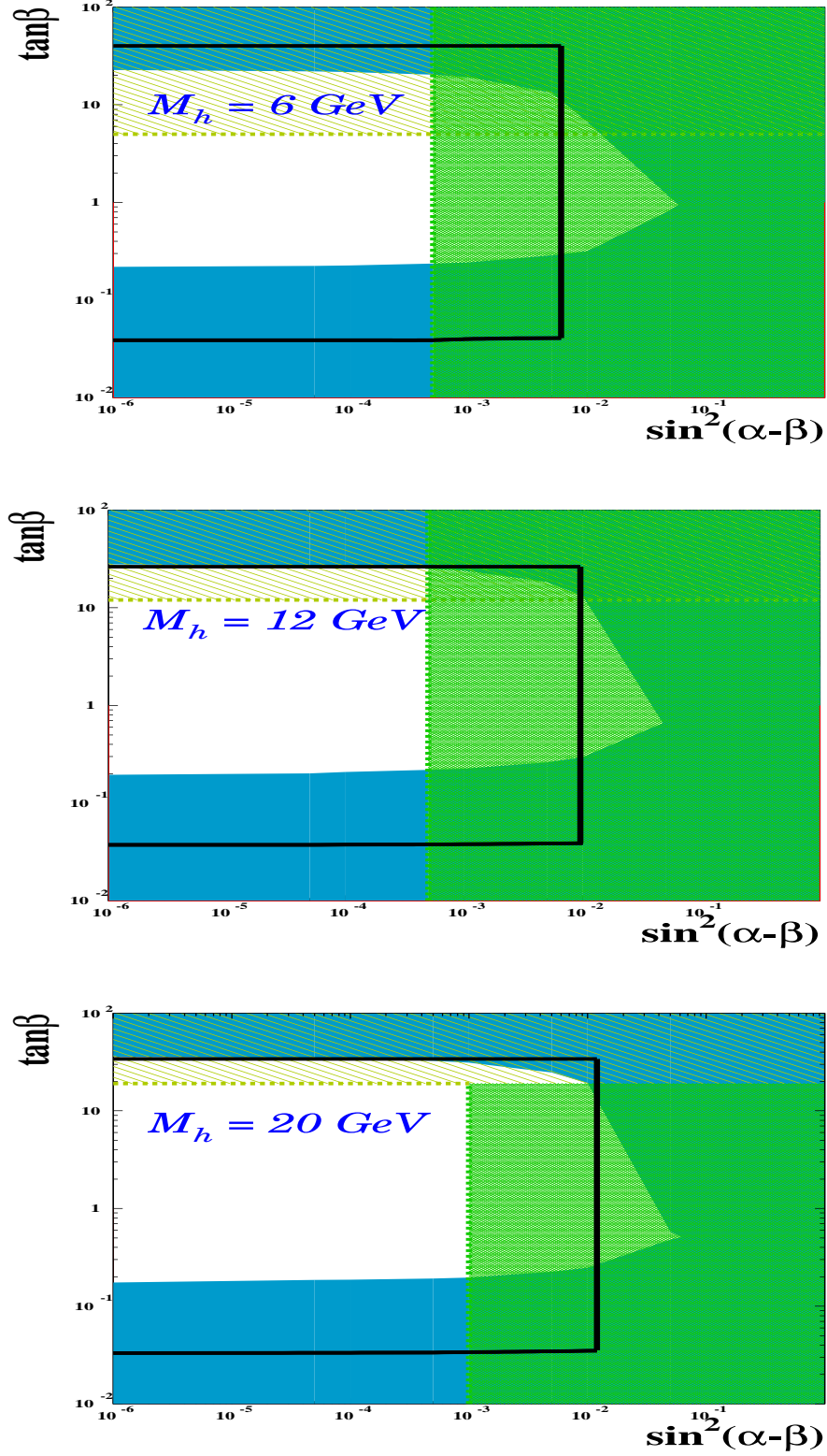
Figure 1: Limits on \sin^2(\beta - \alpha) and \tan\beta for a light scalar h of mass M_h = 6, 12 , and 20 \text{ GeV} at GigaZ. The light hatched (yellow) region shows the exclusion from the Yukawa process, the cross hatched (green) region the one from Higgsstrahlung, the dark area depicts the exclusion range from Z \rightarrow \gamma h (with mass of H^\pm = 300 \text{ GeV} ). Also shown are the current best limits from LEP (black line).
