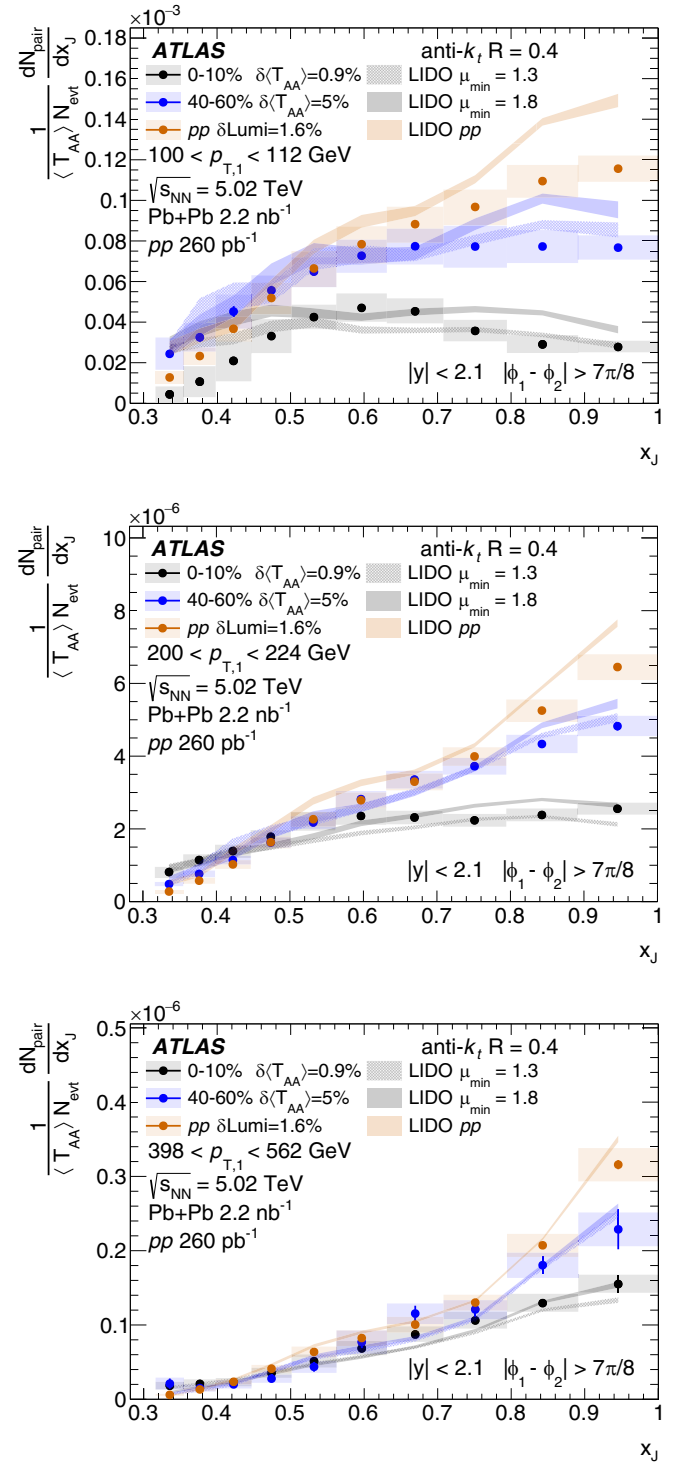
FIG. 12. The absolutely normalized x_j distributions for 100 < p_{T,1} < 112 GeV (top), 200 < p_{T,1} < 224 GeV (center), and 398 < p_{T,1} < 562 GeV (bottom) in Pb+Pb collisions. For Pb+Pb collisions, the measurements are compared with predictions from LIDO [42] for two values of the jet-medium coupling cutoff parameter, \mu_{\min} = 1.3 and \mu_{\min} = 1.8 , and the pp collision measurements are compared with the LIDO pp collision calculation.
