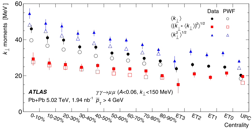
FIG. 21. Moments of the \gamma\gamma \rightarrow \mu^+\mu^- k_\perp distributions as a function of centrality compared with the PWF predictions. The error bars indicate combined statistical and systematic uncertainties. In some bins, the statistical uncertainties, determined both by the number of counts and by their k_\perp distribution, dominate.
