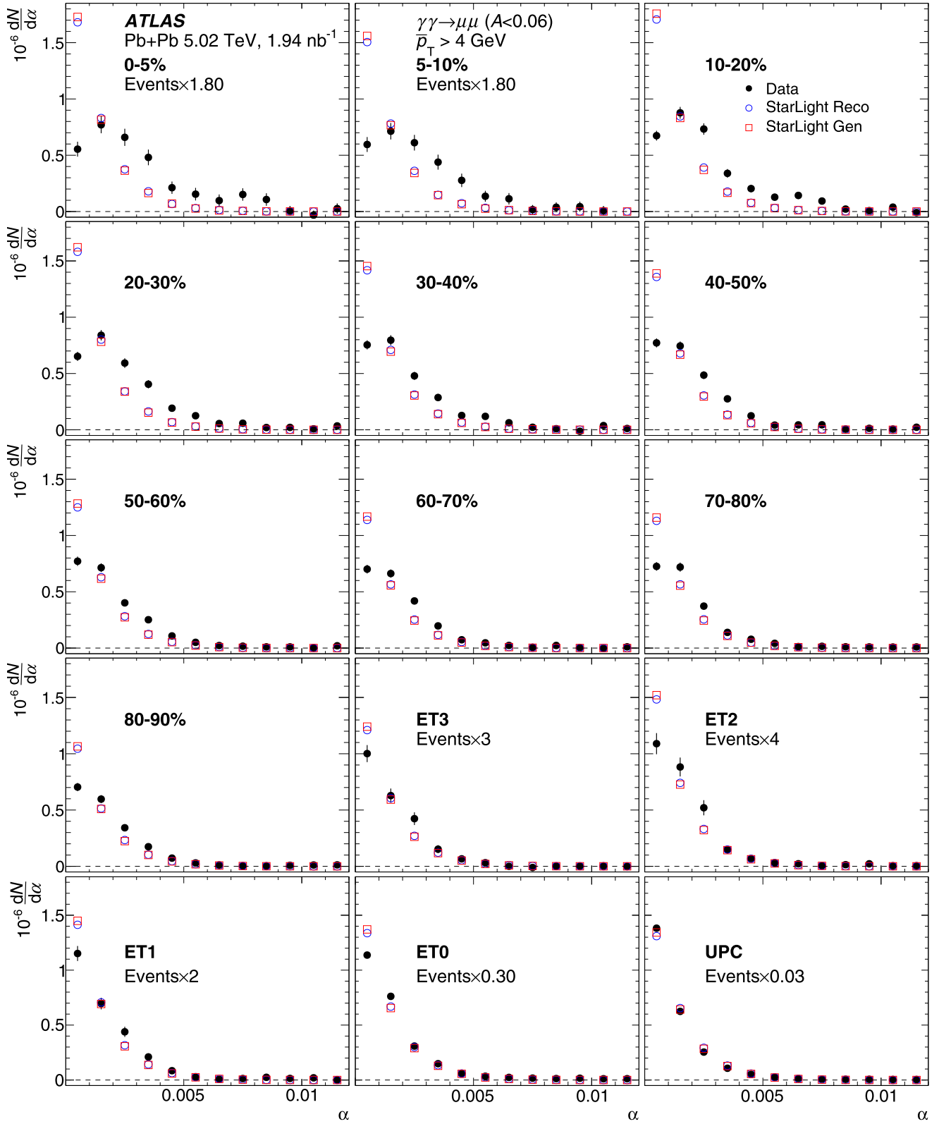
FIG. 11. HF + DY background-subtracted \alpha distributions for pairs satisfying the Fid- \alpha selection and having \bar{p}_T > 4 \text{ GeV} in different centrality intervals from the most central 0–5% (top left) to the UPC interval (bottom right). For a few panels the distributions are scaled to allow a common y-axis range for the plots. The scale factors are stated on the panels. Also shown for comparison are the generated and reconstructed distributions obtained from the STARlight simulation samples. The STARlight generated and reconstructed distributions are scaled to match the corresponding data distributions over the \alpha < 0.012 interval.
