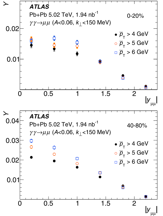
FIG. 17. Measured normalized yields of \gamma\gamma \rightarrow \mu^+\mu^- pairs passing the Fid- k_\perp selection as a function of the pair rapidity, |y_{\mu\mu}| . The widths of the |y_{\mu\mu}| intervals along the x axis are 0.4 units. The top and bottom panels correspond to the 0-20% and 40-80% centrality intervals, respectively. The error bars indicate statistical (lines) and systematic (shaded boxes) uncertainties. For the 40-80% interval, both sets of errors are typically smaller than the symbols.
