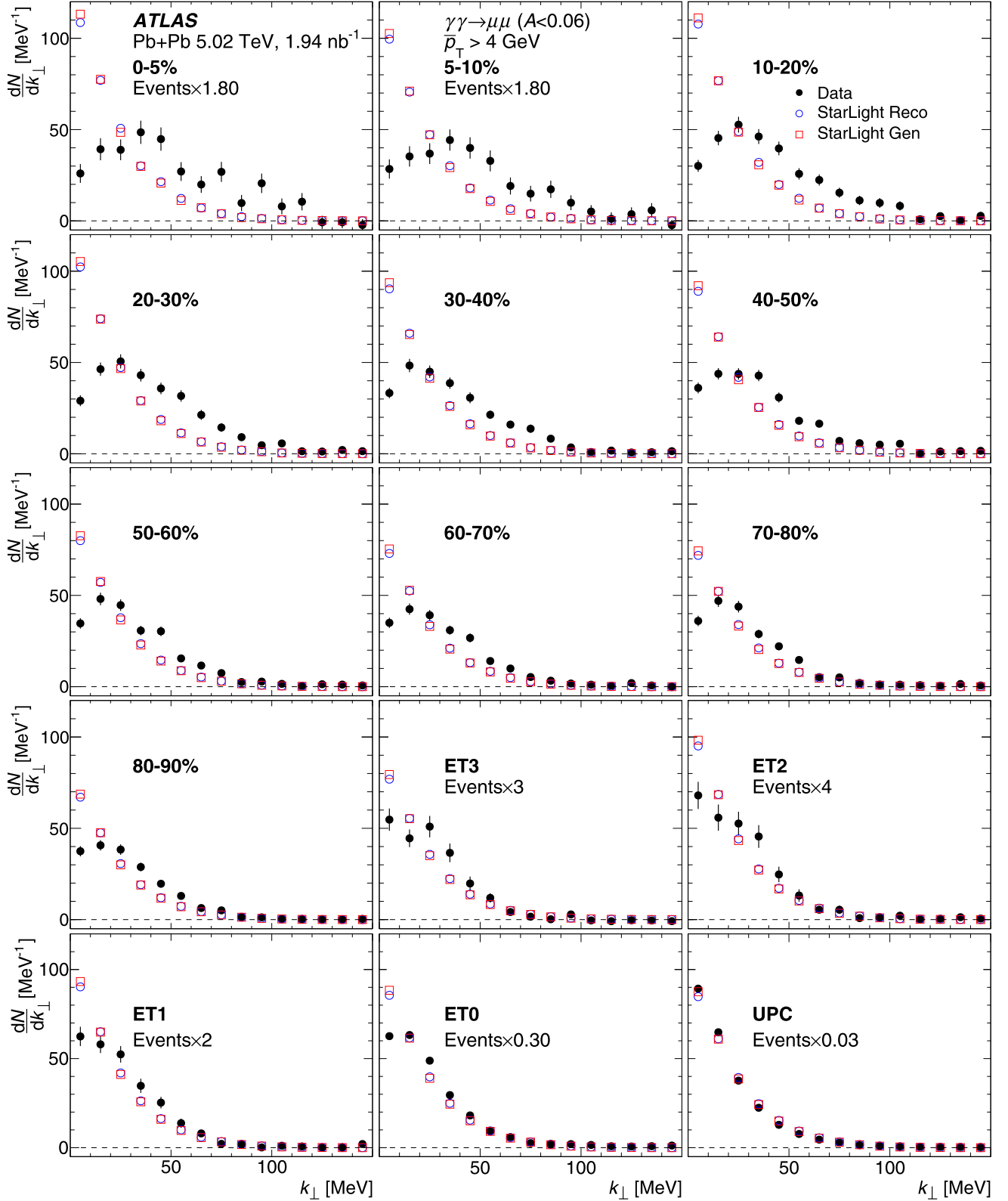
FIG. 12. HF + DY background-subtracted k_{\perp} distributions for pairs satisfying the Fid- k_{\perp} selection and having \bar{p}_T > 4 GeV in different centrality intervals from the most central 0–5% (top left) to the UPC interval (bottom right). For a few panels the distributions are scaled to allow a common y-axis range for the plots. The scale factors are stated on the panels. Also shown for comparison are the generated and reconstructed distributions obtained from the STARlight simulation samples. The STARlight generated and reconstructed distributions are scaled to match the corresponding data distributions over the k_{\perp} < 150 MeV interval.
