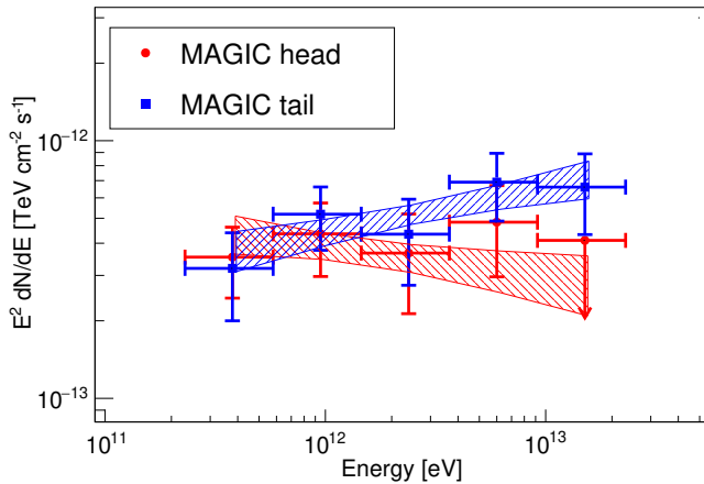
Fig. 3. Energy spectra of the head and tail regions. Red and blue data represent the spectra of the head and tail, respectively. The color ‘bow-tie’ areas show the result of fitting with a simple power-law function and 1\sigma statistical uncertainties.
