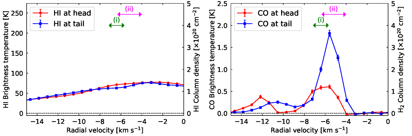
Fig. B.1. HI (left) and ^{12}\text{CO} ( J = 1 - 0 ) (right) radial profile at the head and tail region. In both panels, red and blue data represent the profile of the head and tail regions. The green arrow labelled (i) show the velocity ranges pointed out by Kothés et al. (2001) , while the magenta arrow labelled (ii) is those of Acciari et al. (2009) and Albert et al. (2020) .
