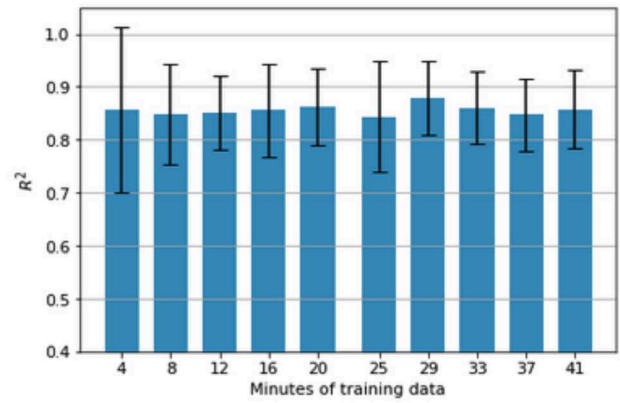
Figure 4: Average R^2 for the eight predicted outputs with varying amounts of training data
