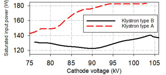
Figure 5: Saturated input power versus cathode voltage for two klystrons types used at XFEL.
