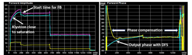
Figure 6: Klystron input (yellow) and output (blue and magenta) amplitude and phases waveforms. Phase and amplitude compensation for rise and fall times only.
