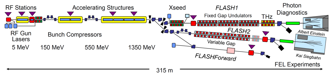
Figure 3. FLASH layout.
