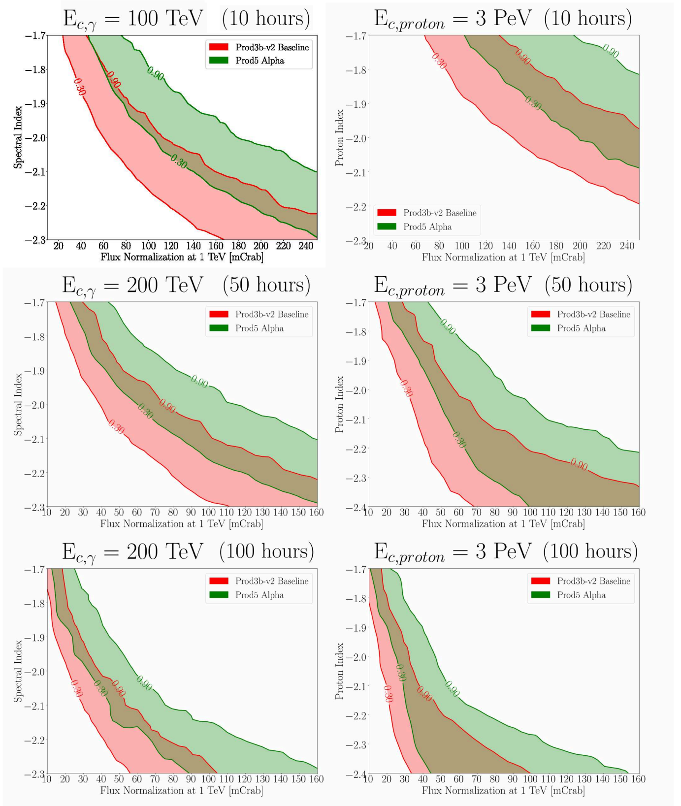
Figure D.16: Comparison of "transition regions", i.e. the regions between 30% and 90% detection probability, for the detection of a true spectral \gamma -ray cutoff (left panels) and the detection of a true PeVatron with a hadronic spectral cutoff at 3 PeV (right panels) after 10 (top), 50 (middle) and 100 (bottom) hours of observation. The "transition regions" shown as red and green shaded areas are obtained by using "Prod 3b-v2" (Baseline) and "Prod 5-v0.1" (Alpha) IRFs, respectively.
