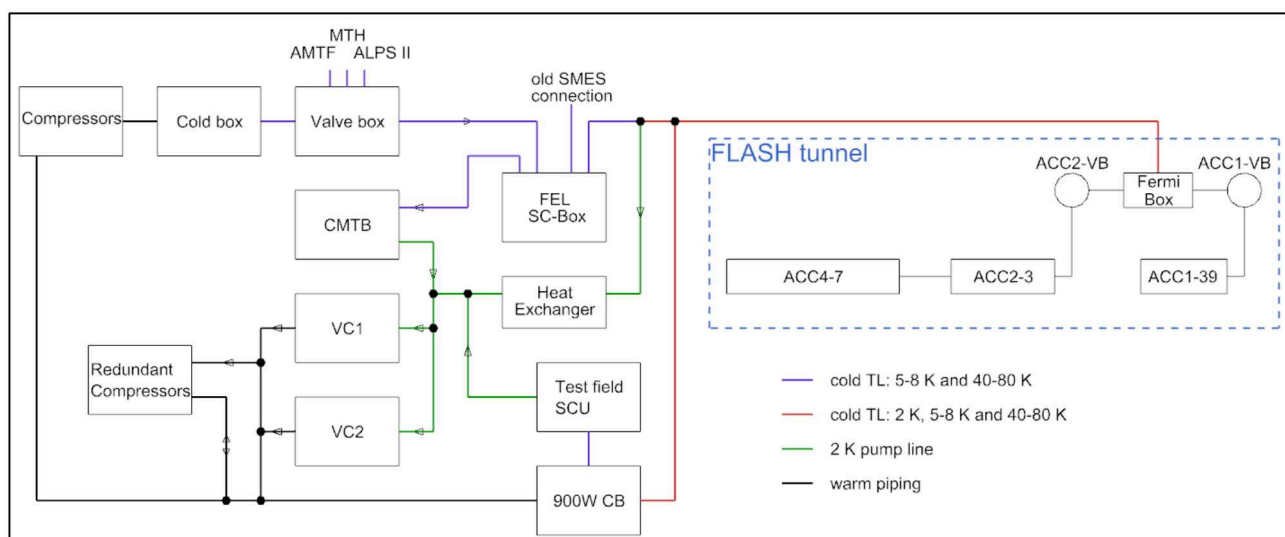
Figure 3: Schematic layout of FLASH cryogenic.
