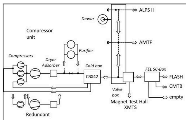
Figure 4: Layout of the FLASH cryoplant.
