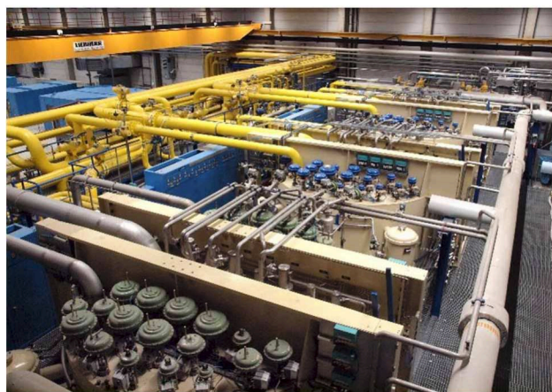
Figure 5: The cryoplant cold boxes.
