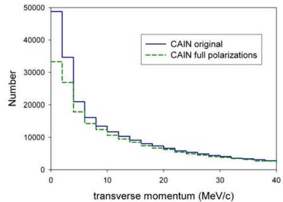
Figure 7: Transverse momentum of final pairs.
