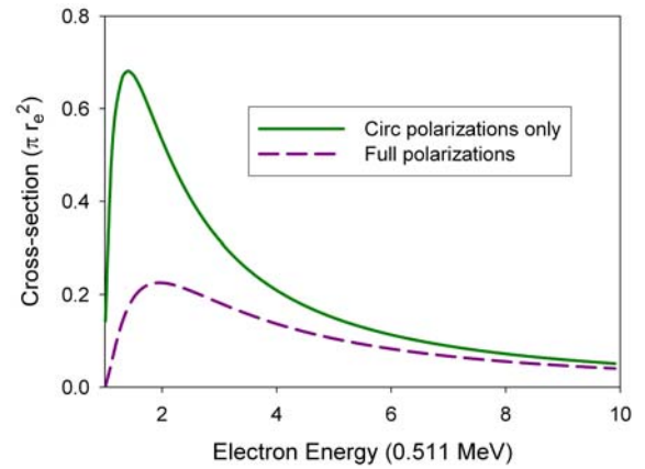
Figure 3: Breit-Wheeler cross-section.
