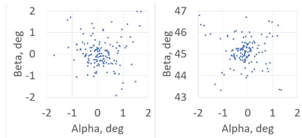
Figure 5. Error distribution of the magnetisation axis for magnets A (left) and B (right) as a result of Helmholtz coil characterization.
