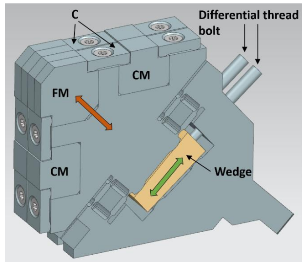
Figure 8. Keeper design. FM: function magnet, CM: compensation magnet, C: clamps. The wedge is moved by turning the differential thread bolt. Its movement along the direction indicated by the green arrow will move the function magnets in the direction of the brown arrow, towards or away from the beam.
