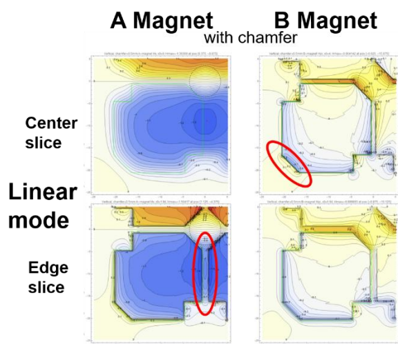
Figure 6. Demagnetising fields for A and B magnets in linear mode. Areas with strong demagnetisation effects are highlighted by red circles. On the colour scale dark blue and dark orange represent extremal positive and negative values, respectively, while white corresponds to zero.
