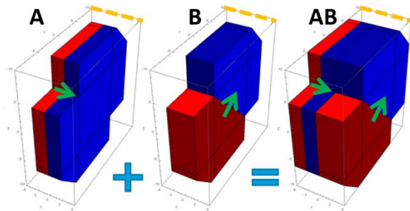
Figure 4. Magnets A and B. Green arrows indicate the direction of magnetisation; the dashed orange line represents the beam axis. Magnets will be glued together to form AB- or BA-pairs.
