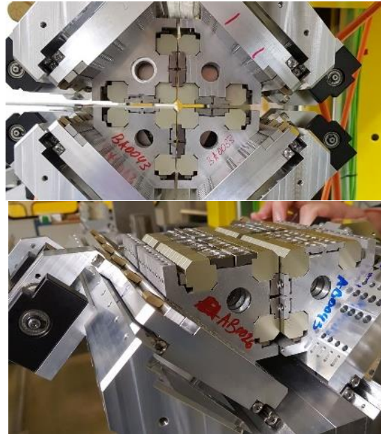
Figure 2. Pictures of the APPLE-III prototype. Top: View along the beam axis. Bottom: Bottom structure.
