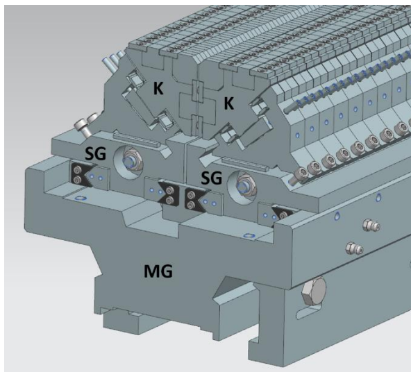
Figure 7. Design of the girder structure and keepers. MG: Main girder, SG: sub-girder, K: keeper.
