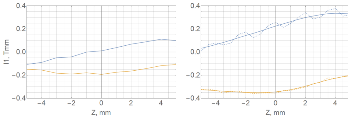
Figure 3. First field integral vs transverse position from measurements of the assembled prototype structure (left) and from simulations based on measurements of the individual keepers (right). Blue: vertical component, yellow: horizontal component. The dashed lines in the graph on the right show some systematic errors of the measurement system which is visible only when 32 individual measurements are summed up for prediction.
