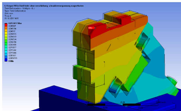
Figure 9. Deformation of the keeper. Colour scale ranges from 0 (dark blue) to 0.053 mm deformation (red) on a linear scale.
