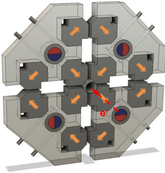
Figure 1. Arrangement of magnets in the APPLE prototype. Orange arrows indicate direction of magnetisation of the permanent magnets.
