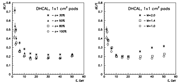
Fig. 2. Energy resolution of the DHCAL as a function of energy: (left) for different efficiencies; (right) for different fired pad multiplicities.
