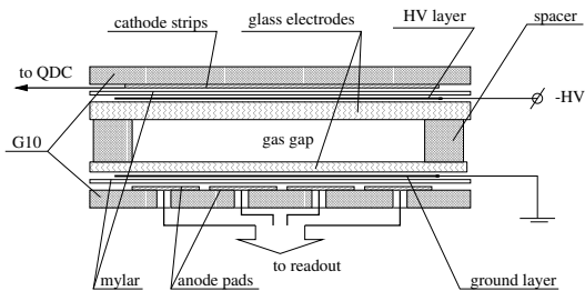
Fig. 3. Schematic cross section of RPC prototypes.
