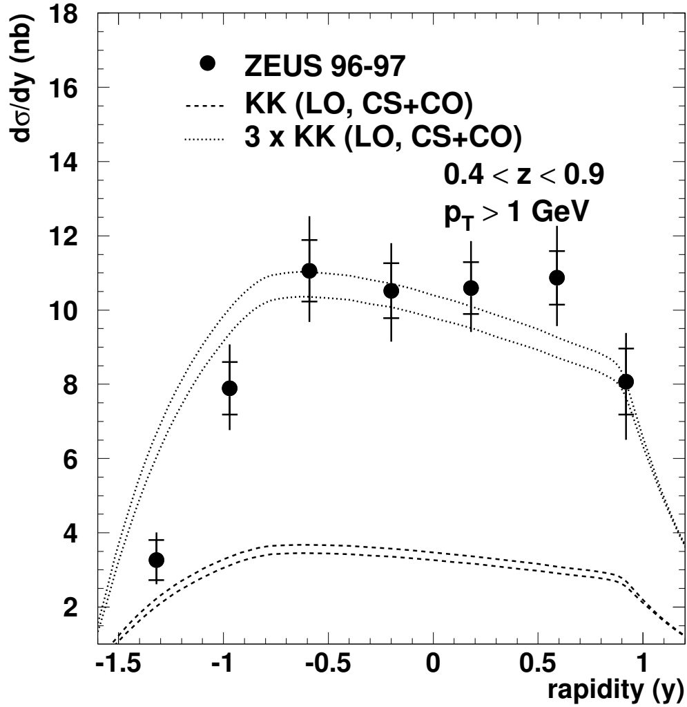
Figure 10: J/\psi differential cross-section d\sigma/dy for 50 < W < 180 GeV, 0.4 < z < 0.9 and p_T > 1 GeV. The inner error bars show the statistical uncertainty; the outer bars show the statistical and systematic uncertainties added in quadrature. The range of the KK (LO, CS+CO) prediction is shown as the dashed lines. The dotted lines show the same prediction scaled up by a factor of three. The spread in the predictions is due to theoretical uncertainties in the extraction of the CO matrix elements. A 15 % contribution has been added to the predictions to account for J/\psi mesons originating from \psi' cascade decays.
