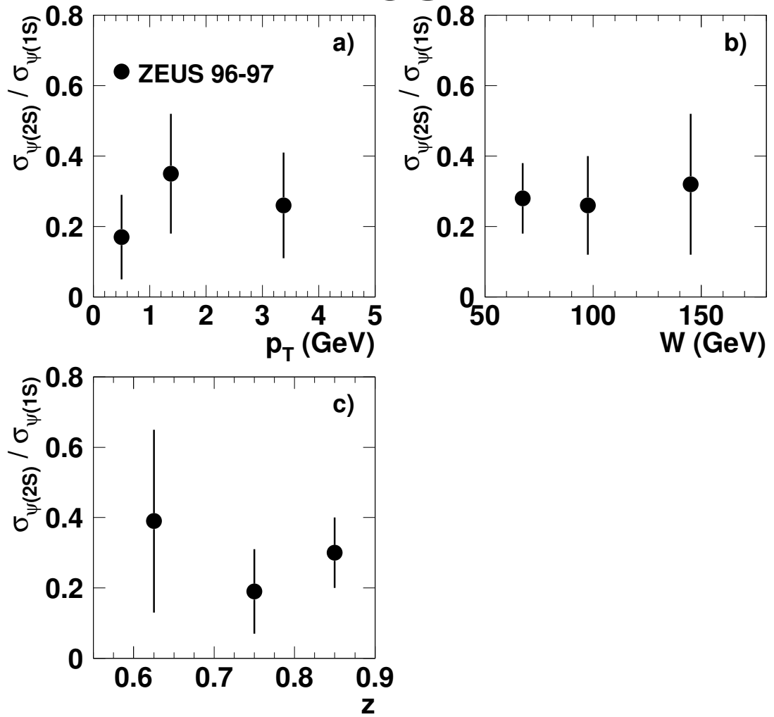
Figure 4: \psi' to J/\psi cross-section ratios as a function of a) p_T , b) W , and c) z , measured for 50 < W < 180 GeV and 0.55 < z < 0.9 . The uncertainties are statistical only.
