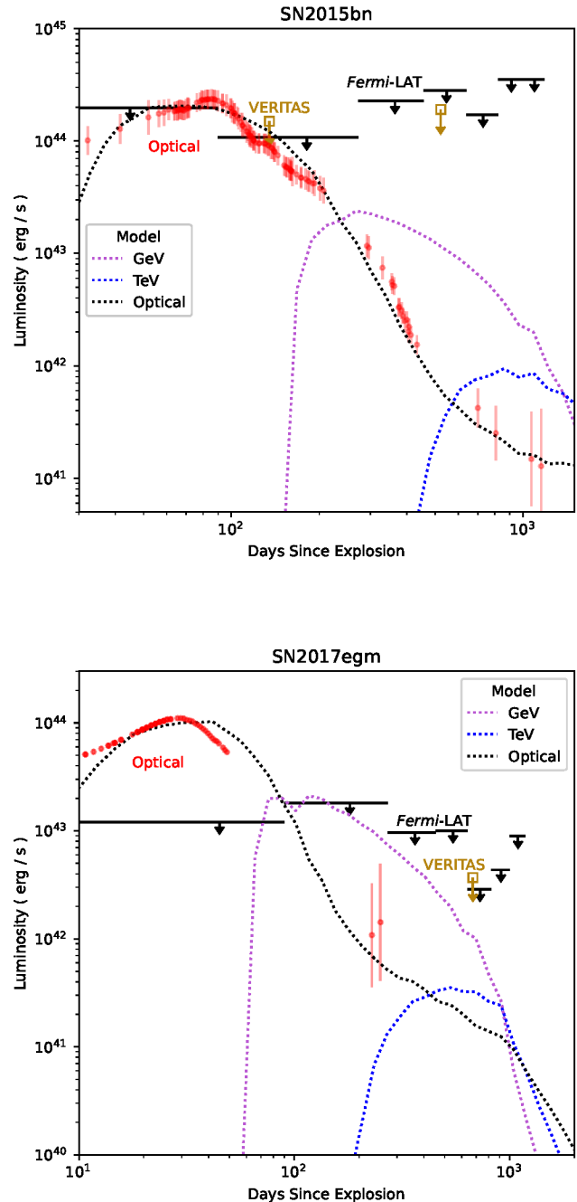
Figure 4. Model light curve for nebular magnetization (from Vurm & Metzger (2021)) for SN2015bn with \epsilon_B = 10^{-7} (top panel) and SN2017egm with \epsilon_B = 10^{-6} (bottom panel).
