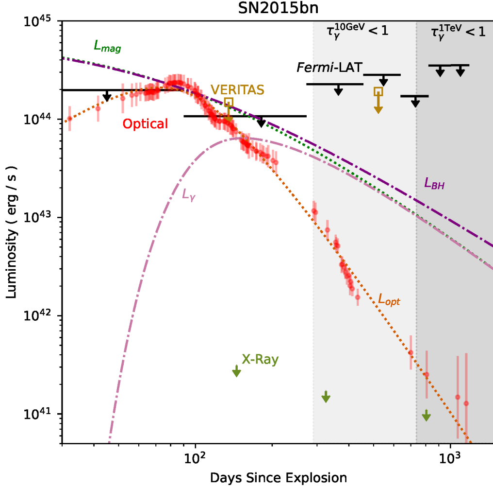
Figure 2. Light curves of SN2015bn spanning 30-1500 days after explosion. Curves shown include (1) the (thermal) supernova luminosity, L_{opt} , fit to UVOIR bolometric luminosity data (in red; Nicholl et al. 2018) to obtain the magnetar parameters; (2) magnetar spin-down luminosity, L_{mag} (green dotted line); and (3) predicted gamma-ray luminosity that escape the ejecta, L_{\gamma} (pink dotted-dashed line; Equations A1, A3 and A4). Black bars show Fermi -LAT upper limits reported for six 180 day bins starting \sim 90 days after explosion. The olive open box shows the VERITAS integral energy flux
