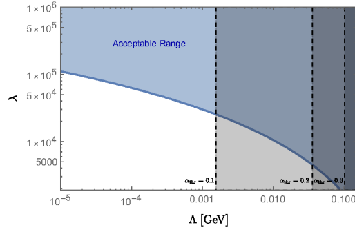
Figure 6. Region of the parameter space \{\lambda, \Lambda\} that allows to reproduce the correct axion DM relic density. The blue shaded region ensures that the QCD axion does not roll until T_{\text{crit}} at which time the dark sector is spontaneously broken. Finally the gray shaded regions signal the parameter space for which our expressions for the thermal friction breakdown before T_{\text{crit}} is reached for different options of the threshold value of the running coupling.
