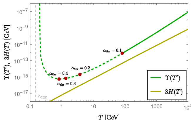
Figure 4. Gauge friction versus Hubble friction for some example parameter values. The red dots denote the instant we switch off the friction effects depending on the largest acceptable value of the gauge coupling \alpha_{\text{thr}} .
