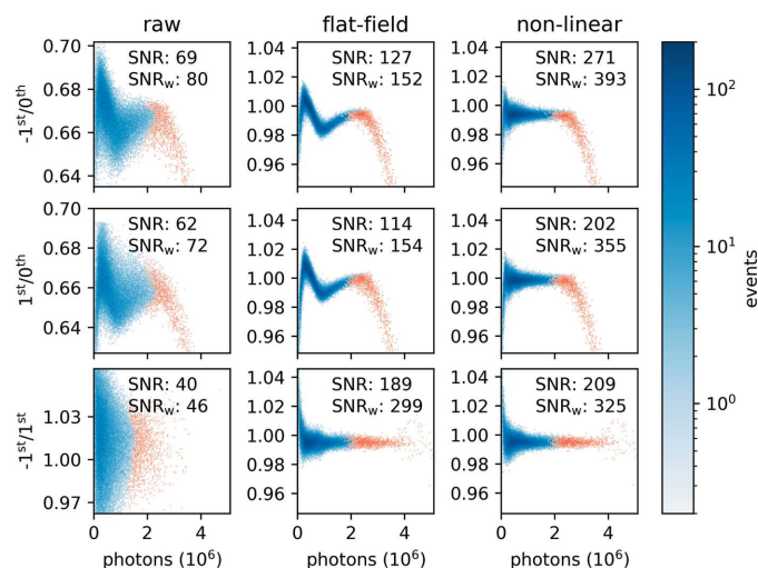
Figure 5 Two-dimensional histograms of the three ratios (-1st/0th grating order in the top row, 1st/0th in the middle row, and -1st/1st in the bottom row) as a function of the number of photons in the 0th order for dark-corrected data in the left 'raw' column, for the dark-corrected and flat-field-corrected data in the middle 'flat-field' column, and finally for the dark-corrected, flat-field-corrected and non-linear-corrected data in the right 'non-linear' column. Data that contain saturated pixels are shown as red, as opposed to blue where no saturation occurs. In each plot, the SNR and weighted SNR ( \text{SNR}_w ) of the non-saturated events are indicated.
