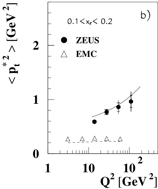
Figure 8: \langle p_t^{*2} \rangle in two intervals of x_F as a function of a) W and b),c) Q^2 compared with results from \mu p DIS experiments (EMC [5] and E665 [48]). The prediction of the MEPS Monte Carlo calculation is compared with the results of this analysis (solid line) and of [5] (dashed line).
