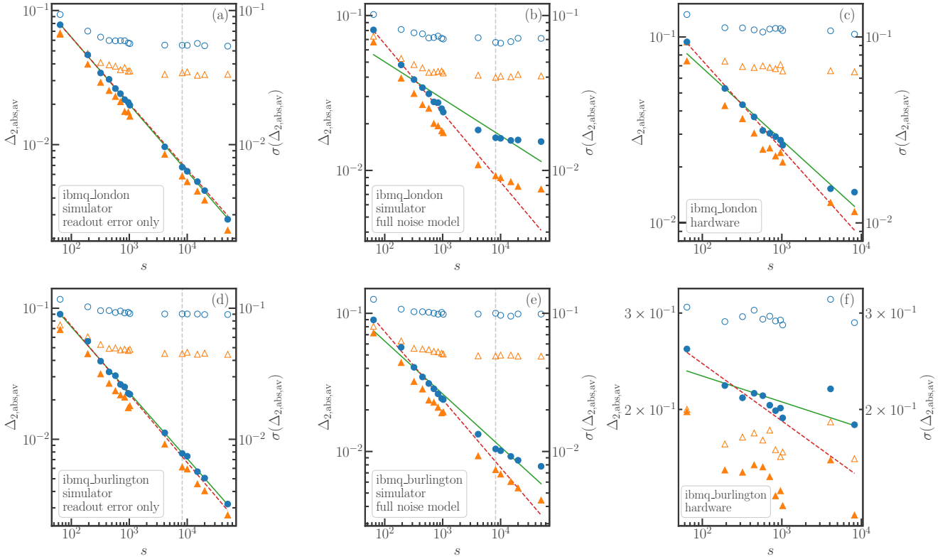
FIG. 6. Mean value \Delta_{2,\text{abs},\text{av}} (blue dots, left y-axes) and standard deviation \sigma(\Delta_{2,\text{abs},\text{av}}) (orange triangles, right y-axes) of the absolute error in Eq. (42) after applying the correction procedure (filled symbols) and without it (open symbols) as a function of the number of shots s . The panels in the upper row correspond to data obtained for ibmq_london , the panels in the lower row to data obtained for ibmq_burlington . The different columns correspond to a classical simulation of the quantum device taking into account only readout error (first column), the full hardware noise model (second column), and data obtained on actual quantum hardware (third column). The solid green lines correspond to a power-law fit to all our data points for the mean absolute error, while the red dashed lines correspond to a fit including the lowest four number of shots. The vertical gray dashed lines in panels (a),(b) and (d),(e) indicate the maximum number of shots that can be executed on the actual hardware.
