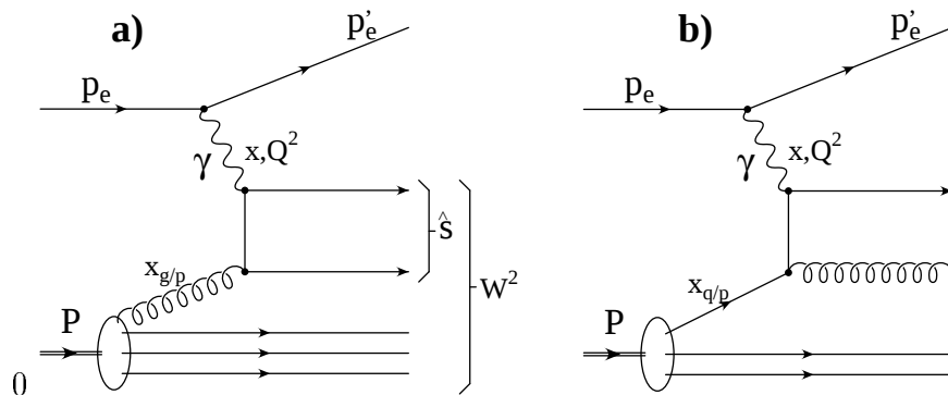
Figure 1: Generic Feynman diagrams for a) the boson-gluon fusion process and, b) the QCD-Compton process
