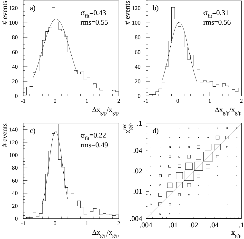
Figure 3: The relative error in the reconstruction of the fractional gluon momentum, \Delta x_{g/p}/x_{g/p} , where \Delta x_{g/p} = x_{g/p}^{\text{rec}} - x_{g/p} , for BGF events generated by the MEPS model. In a) equation (2) has been used, in b) equation (3) and in c) the combination of the two. The correlation between the reconstructed and true x_{g/p} for the combined method is shown in d).
