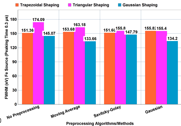
Figure 4. Results of several digital signal processing methods.
