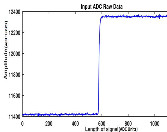
Figure 7. ADC Data for a single photon. Figure 8. Results of several digital signal processing methods.
