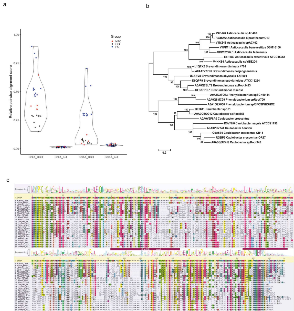
Figure 7. Sequence alignment and distance of SmbA homologs. (a) Pairwise Needleman-Wunsch global alignment scores of SmbA and CckA reciprocal best BLAST hits (BBH) for species sampled from prostheteate Caulobacterales (PC), non-prostheteate Caulobacterales (NPC), and other bacterial groups (OG). Alignment scores are reported relative to self-alignment of SmbA (Q9A5E6) and CckA (H7C7G9) from Caulobacter crescentus . For the null models, CckA BBH was scored against SmbA and vice versa. The latter BBH was identified using BLASTp against the NCBI-NR database using the BLOSUM45 scoring matrix. (b) A phylogenetic tree of 24 SmbA orthologs inferred using the Maximum Likelihood method based on the JTT model as implemented in MEGA7. Branch lengths indicate the number of substitutions per site. The tree with the highest log likelihood (−9134.38) is shown, with bootstrap support from 100 replicates indicated at branches. (c) Sequence alignment and logo of SmbA orthologs. The sequence logo was generated using the WebLogo server from the global alignment of SmbA orthologs used to build the distance tree.
