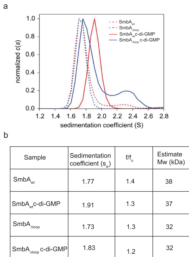
Figure 4. Analytical ultracentrifugation (AUC) analysis of SmbA_{wt} and SmbA_{\Delta loop} . (a) SV-AUC absorbance c(s) distributions of SmbA_{wt} , SmbA_{wt}/(c\text{-di-GMP})_2 , SmbA_{\Delta loop} and SmbA_{\Delta loop}/c\text{-di-GMP} . (b) Mass estimation and s and f/f_0 values of SmbA_{wt} , SmbA_{wt}/(c\text{-di-GMP})_2 , SmbA_{\Delta loop} and SmbA_{\Delta loop}/c\text{-di-GMP} .
