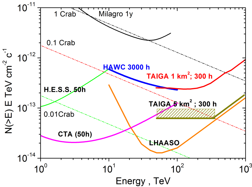
Fig. 6. Sensitivity of the TAIGA experiment for 300 hours of observations in hybrid mode (without muon detectors). A comparison to sensitivities of other experiments is not straight forward, since also the angular and spectroscopic resolutions play an important role for measurements of the morphology and spectra of astrophysical objects. TAIGA has a relative energy resolution of better than 20% and an angular resolution of the order of 0.1°.
