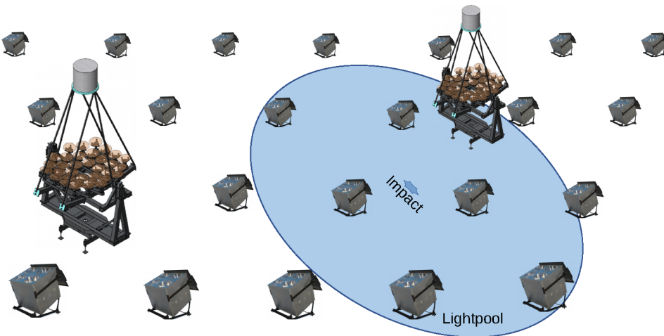
Fig. 4. Schematic drawing of the principle of hybrid operation.
