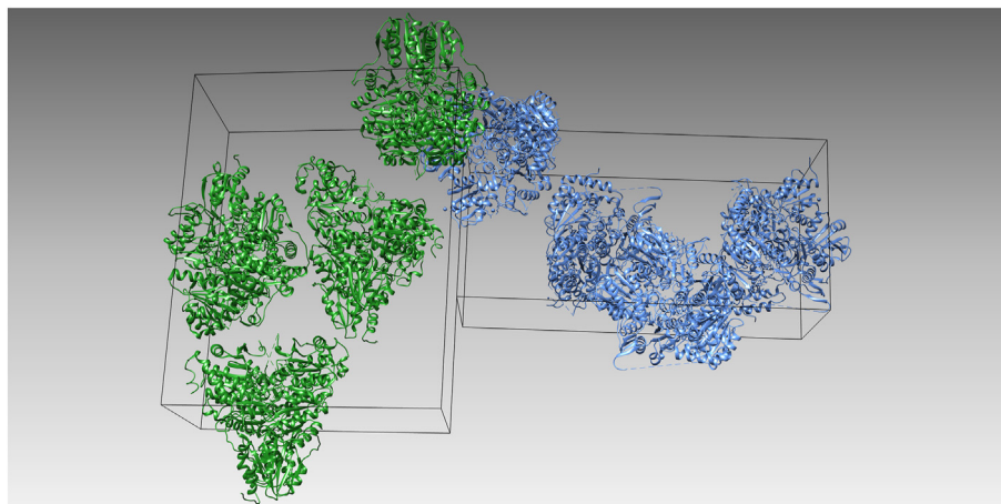
Fig. 3. Left, green: Unit cell of the drDXS enzyme in the 2o1x and 6ouu crystal structures. Cell size is 78 \times 125 \times 151 Å with a volume of 1.47 \times 10^6 Å 3 ; right, blue: Unit cell of ΔdrDXS. Unit cell parameters are with 72 \times 87 \times 181 Å resulting in a smaller volume of 1.13 \times 10^6 Å 3 . (For interpretation of the references to color in this figure legend, the reader is referred to the Web version of this article.)
