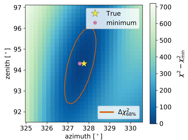
Fig. 10 Same as Fig. 9 (top panel), but for a high-quality event with large contribution in the Hpol antennas
