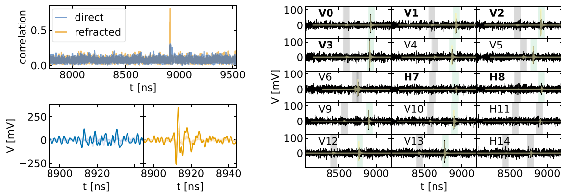
Fig. 2 The pulse selection procedure. Left, top: the total template correlation for the phased array antennas for each ray-type hypothesis ('direct' or 'refracted'/reflected'), indicating here a better correlation for refracted. Left, bottom: The individual as well as coherently-summed (beamformed) pulses for each ray type. Right: Window selection for both ray types. The pulse windows to include in the fit are
