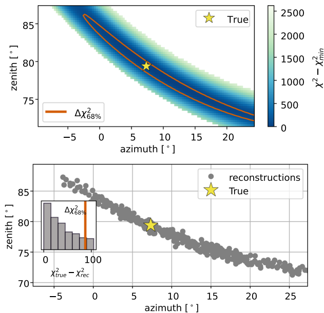
Fig. 12 Same event as Fig. 9, including systematic uncertainties
