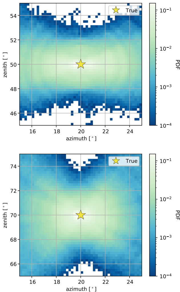
Fig. 11 Top: simulated best-fit points using the obtained resolution for quality cut (H) of the uncertainties in signal direction, viewing angle and polarization for a point source located at zenith of 50^\circ . For details refer to the text. Bottom: same as the top figure, but for a source located at zenith of 70^\circ . Clearly seen is the zenith dependent shape of the point spread function
