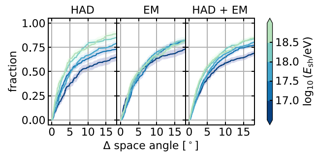
Fig. 5 The space angle distribution for events passing the analysis cut, for different shower types and energies. For hadronic events, high-energy showers in general give higher amplitude signals, leading to an improving resolution as a function of energy
