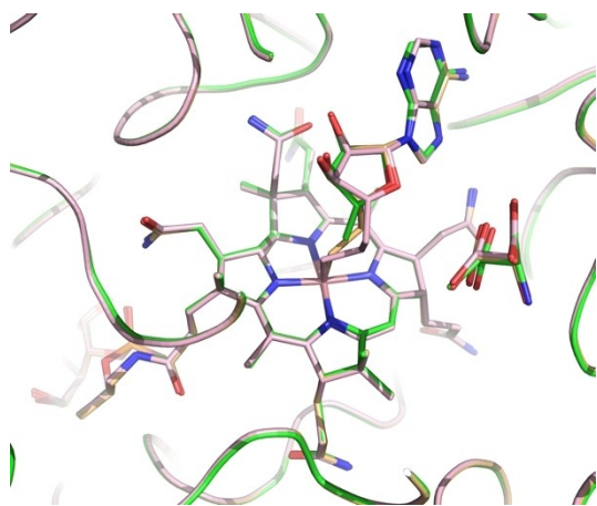
Figure 5. Superposition of active site structures of GM reconstituted with AdoCbl (green, r_s -conf), AdoMeCbl (orange), and AdoEtCbl (pink), highlighting stick-models of the bound homologous AdoCbls, the substrate 3-methylaspartate (green), and the pseudo-substrate tartrate (pink).
