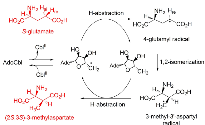
Figure 2. Key radical steps in the reversible isomerisation catalysed by the AdoCoBl-dependent GM depicted in the direction from (S)-glutamate to (2S,3S)-3-methylaspartate.
