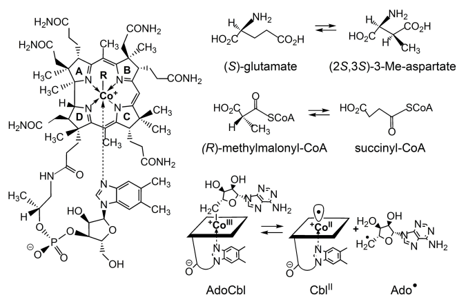
Figure 1. Left: Structural formula of the cobalamins vitamin B 12 (CNCoBl, R = CN), coenzyme B 12 (AdoCoBl, R = 5'-deoxy-5'-adenosyl), methylcobalamin (MeCoBl, R = CH 3 ), cob(II)alamin (Cbl II , R = ε). Right: The carbon skeleton isomerisations catalysed by GM and MCM, and depiction of the Co–C bond homolysis of AdoCoBl that generates the catalytically active 5'-deoxy-5'-adenosyl-radical (Ado•) and Cbl II reversibly.
