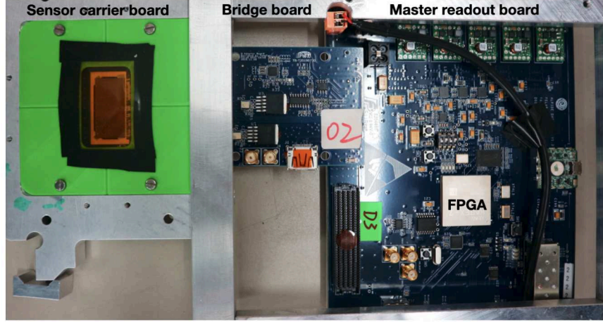
Figure 1: An assembled readout electronic of a telescope plane showing sensor carrier board, bridge board and main readout board.
