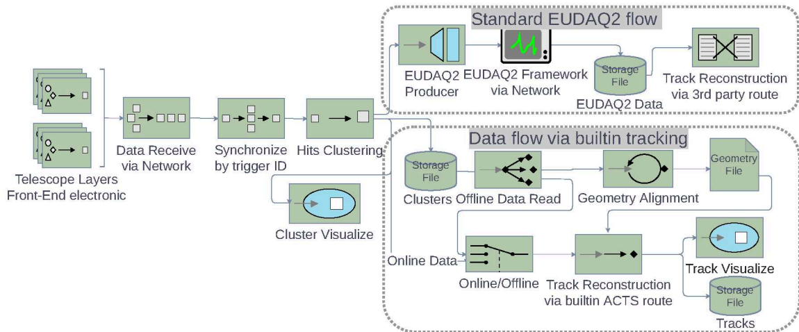
Figure 2: The data flow in ADENIUM from the individual sensor planes to the the user analysis.
