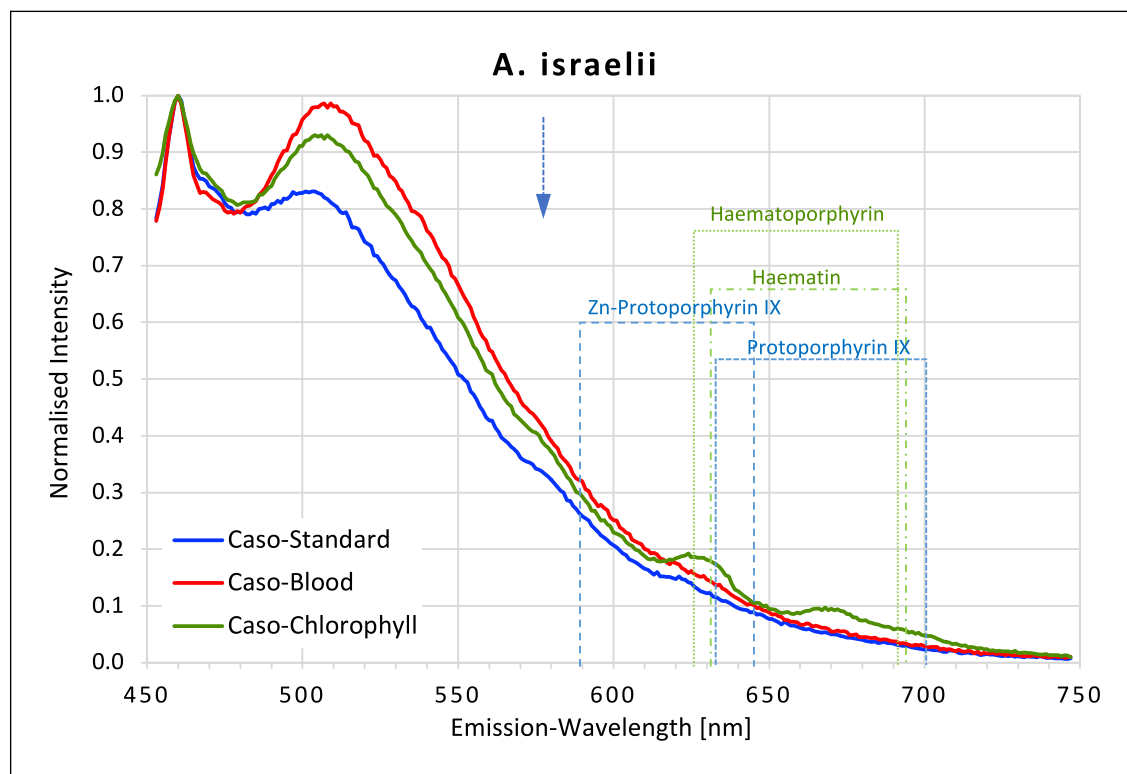
Fig. 3. Fluorescence emission spectra for A. israelii at 405 nm excitation on caso, caso blood, and caso chlorophyll agars. The position of peaks measured for protoporphyrin IX, Zn-protoporphyrin IX, haematoporphyrin, and haematin are shown in dotted lines. Blue arrow at 577 nm.
