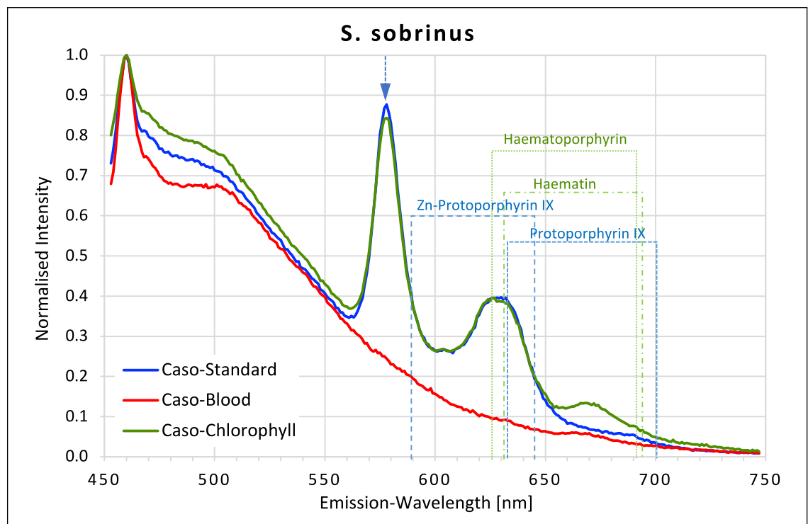
Fig. 10. Fluorescence emission spectra for S. sobrinus at 405 nm excitation on caso, caso blood, and caso chlorophyll agars. The position of peaks measured for protoporphyrin IX, Zn-protoporphyrin IX, haematoporphyrin, and haematin are shown in dotted lines. Blue arrow at 577 nm.
