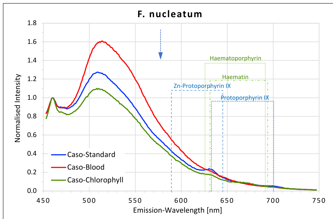
Fig. 5. Fluorescence emission spectra for F. nucleatum at 405 nm excitation on caso, caso blood, and caso chlorophyll agars. The position of peaks measured for protoporphyrin IX, Zn-protoporphyrin IX, haematoporphyrin, and haematin are shown in dotted lines. Blue arrow at 577 nm.
