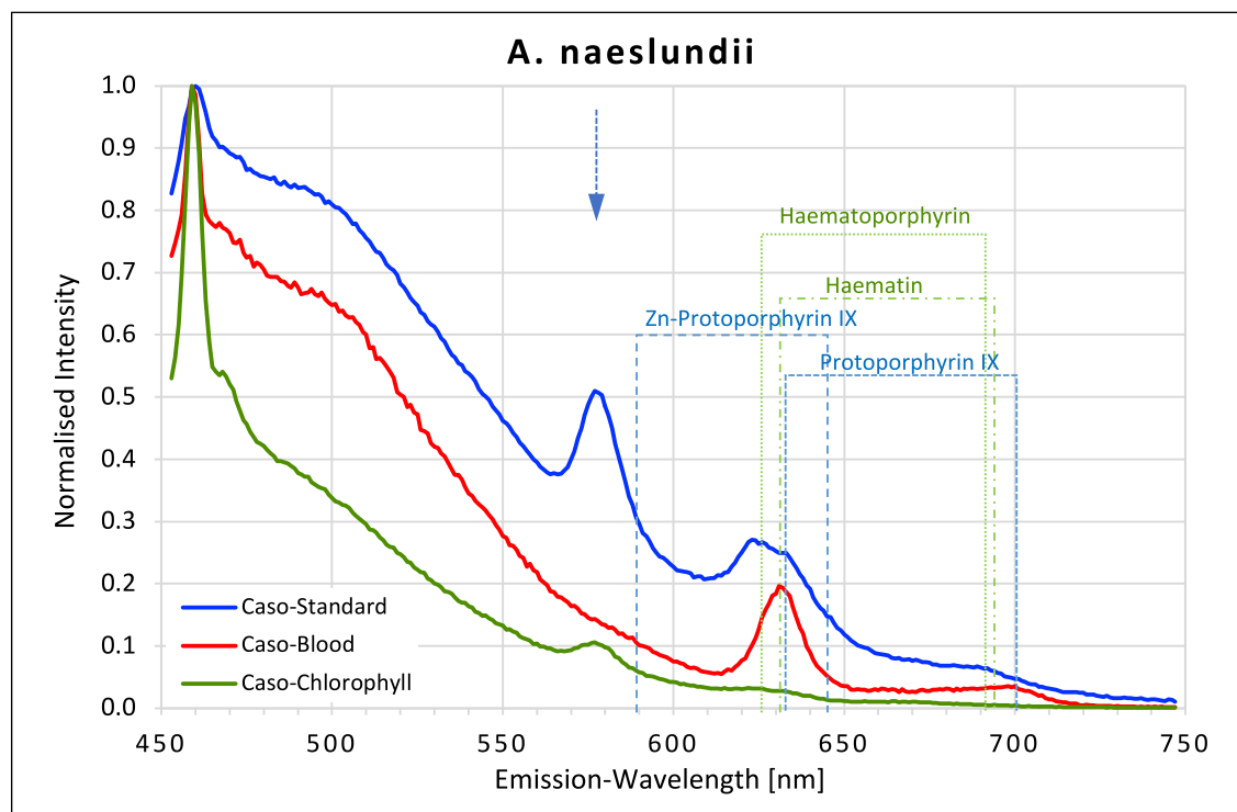
Fig. 4. Fluorescence emission spectra for A. naeslundii at 405 nm excitation on caso, caso blood, and caso chlorophyll agars. The position of peaks measured for protoporphyrin IX, Zn-protoporphyrin IX, haematoporphyrin, and haematin are shown in dotted lines. Blue arrow at 577 nm.
