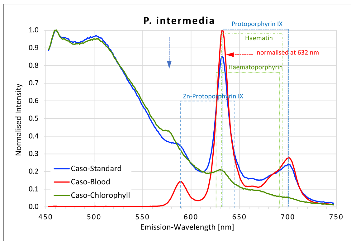
Fig. 2. Fluorescence emission spectra for P. intermedia at 405 nm excitation on caso, caso blood, and caso chlorophyll agars. The intensity on caso blood agar is normalised at 632 nm. The position of peaks measured for protoporphyrin IX, Zn-protoporphyrin IX, haematoporphyrin, and haematin are shown in dotted lines. Blue arrow at 577 nm.
