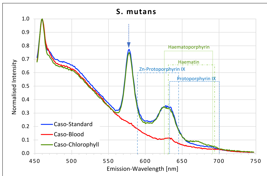
Fig. 7. Fluorescence emission spectra for S. mutans at 405 nm excitation on caso, caso blood, and caso chlorophyll agars. The position of peaks measured for protoporphyrin IX, Zn-protoporphyrin IX, haematoporphyrin, and haematin are shown in dotted lines. Blue arrow at 577 nm.
