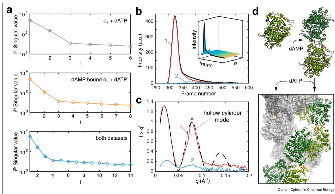
Deconvolution of Bs RNR conformational transition observed by SAXS. a) The singular values (filled in circles) derived from SVD analysis of the titration series of the ligand-free \alpha subunit of Bs RNR with dATP (grey), the dAMP-bound non-canonical \alpha_2 with dATP (orange), and a combination of both datasets (blue). b) SEC-SAXS was performed on the dAMP-bound non-canonical \alpha_2 with a saturating concentration of dATP in the presence of substrate (inset). Two scattering components were deconvoluted by EFA, denoted as 1 & 2 (main plot). c) The major species, 1, shows features of a hollow cylinder model. Panels a–c : adapted under Creative Commons Attribution 4.0 International License [36]. d) Structures illustrating conversion of RNR \alpha monomer (PDB: 6MT9) and dAMP-bound non-canonical \alpha_2 (PDB: 6CGL) to inactive filament (PDB: 6MYX) in the presence of dATP.
