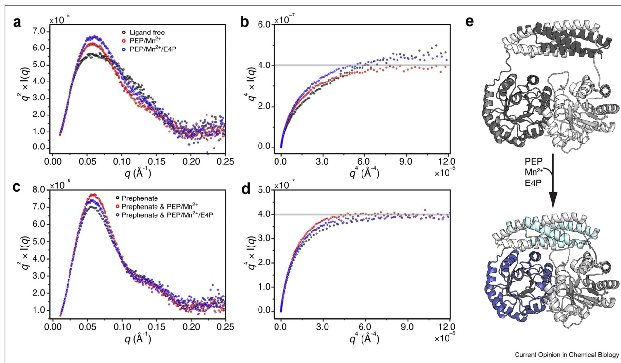
Pn DAH7PS-CM enzyme compaction in response to substrate and product binding. Top panels compare Pn DAH7PS-CM SAXS analysis for ligand-free state (black) with addition of DAH7PS substrates/cofactor, PEP/Mn 2+ (red) or PEP/Mn 2+ /E4P (blue), via a ) Kratky and b ) Porod-Debye plots. The bottom panels demonstrate lack of change when CM product prephenate is bound alone (black), in the presence of PEP/Mn 2+ (red), or PEP/Mn 2+ /E4P (blue), via c ) Kratky and d ) Porod-Debye plots. Panels a–d : adapted under permission (copyright Elsevier, 2021) [15]. e ) AlphaFold2 models of Pn DAH7PS-CM modified to illustrate compaction expected upon DAH7PS substrate binding (not fit to original data).
