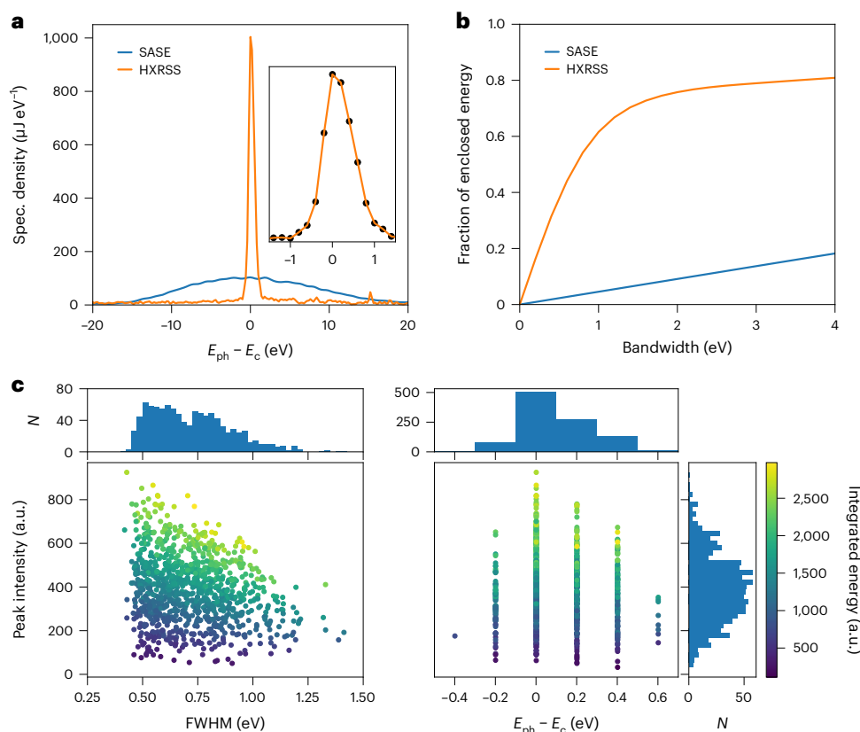
Fig. 2 | HXRSS performance achieved at 9 keV. a , Comparison of the best seeded (HXRSS) pulse (central energy E_c = 9,009.0 eV; average energy, 1.2 mJ; 400 \mu\text{J} background; FWHM bandwidth, 0.8 eV) with typical SASE at the European XFEL (pulse energy, 2.2 mJ; FWHM bandwidth, 20.0 eV). The seeded pulse reaches 1 mJ \text{eV}^{-1} spectral density, obtained by delaying the electron bunches by 45 fs.
