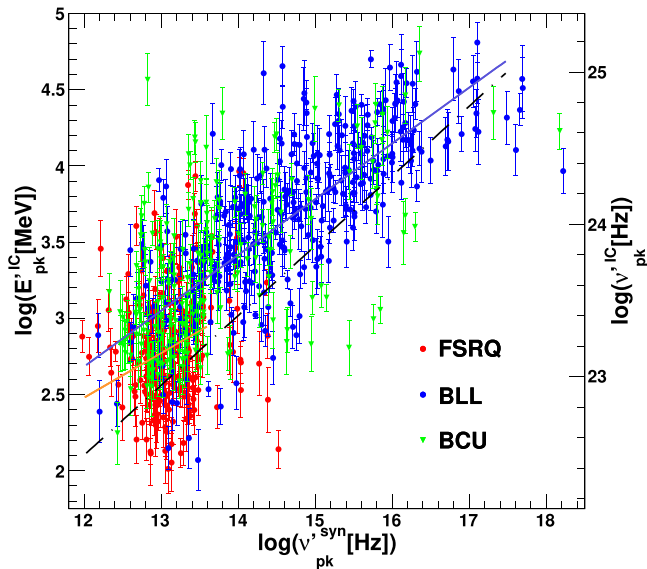
Figure 6. Energy of the high-energy component plotted as a function of \nu'_{pk} , both estimated in the rest frame, for the different blazar classes. The source selection is described in the text. The blue line represents a linear fit to the BL Lac object data and the orange one (restricted to \log(\nu'_{pk}) < 13.6 ) to the FSRQ data. The black dashed-dotted line corresponds to the prescription from Abdo et al. (2010a).
