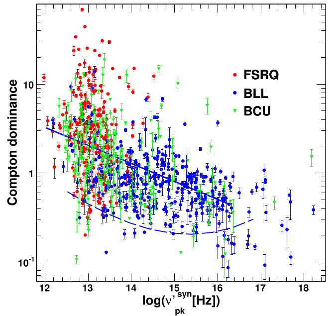
Figure 7. Compton dominance plotted as a function of \nu'_{pk} for the same sources as in Figure 6. The dashed line corresponds to an estimate of the average threshold for BL Lac objects (derived from the threshold plotted in Figure 5) and the solid line to an exponential fit to the BL Lac object data.
