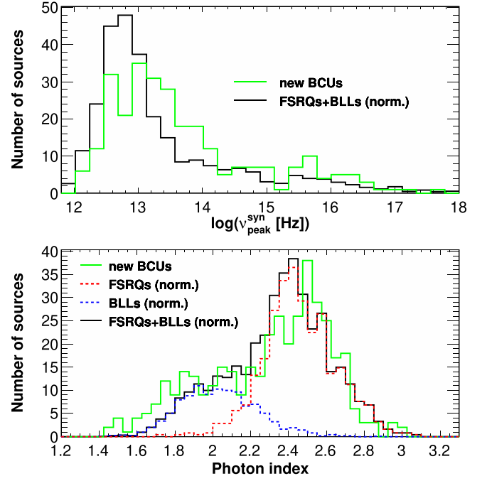
Figure 3. Distributions of \nu_{\text{pk}}^{\text{syn}} (top) and photon index (bottom) of the new (DR2 and DR3) BCUs (green, solid) compared to the arbitrarily normalized sum of the FSRQ and BL Lac object distributions (solid, black). The relative weight between FSRQs and BL Lac objects has been multiplied by 2.5 with respect to that found in 4FGL.
