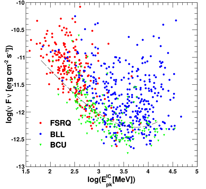
Figure 5. \nu F_{\nu} of the high-energy peak as a function of the peak energy for sources fulfilling the conditions given in the text. Error bars have been omitted for clarity. The dashed curve corresponds to an estimated average threshold.
