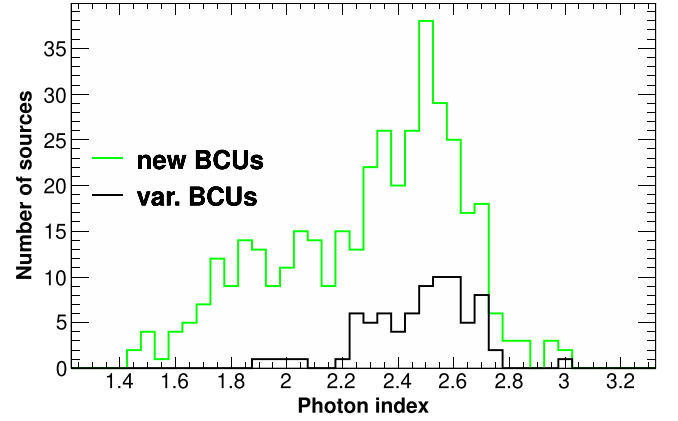
Figure 4. Photon-index distributions for the new BCUs and the subset of sources showing significant variability.
