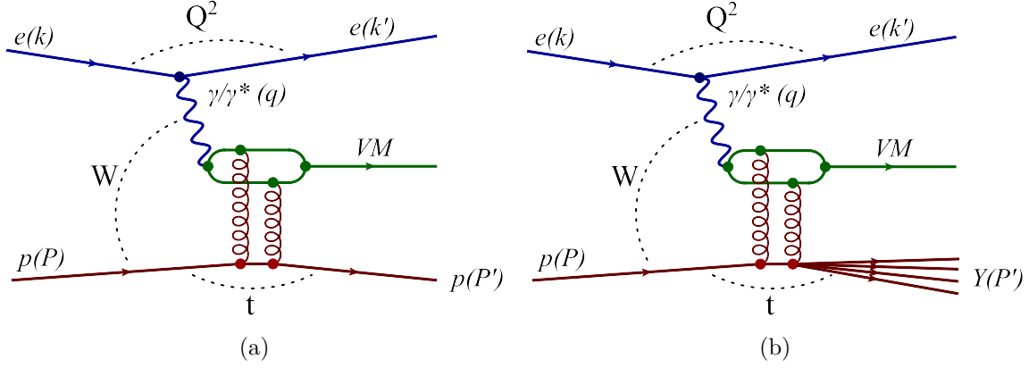
Figure 1. Schematic representation of (a) exclusive and (b) proton-dissociative vector-meson production in ep scattering. For a description of the kinematic variables, see section 1.
